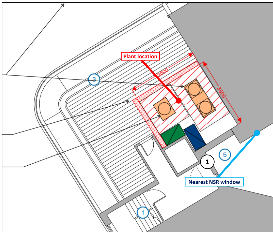
Figure 2.3 Site measurement position and propose plant installations (Image Source: Innovo Engineering Consultancy)
