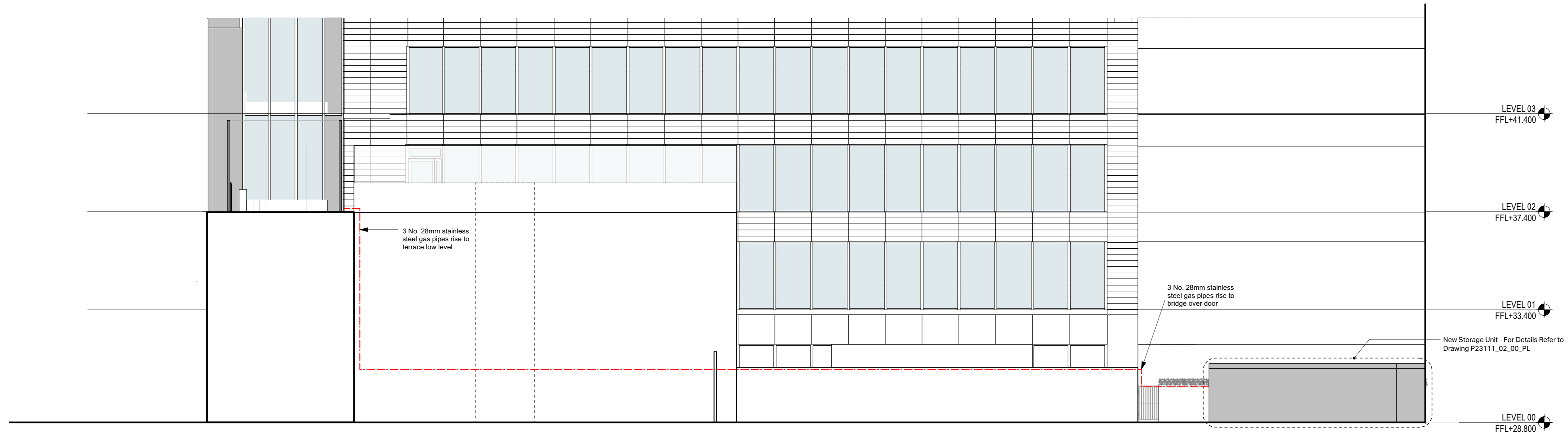
2 Proposed Long Elevation showing pipe route Scale: 1:100
