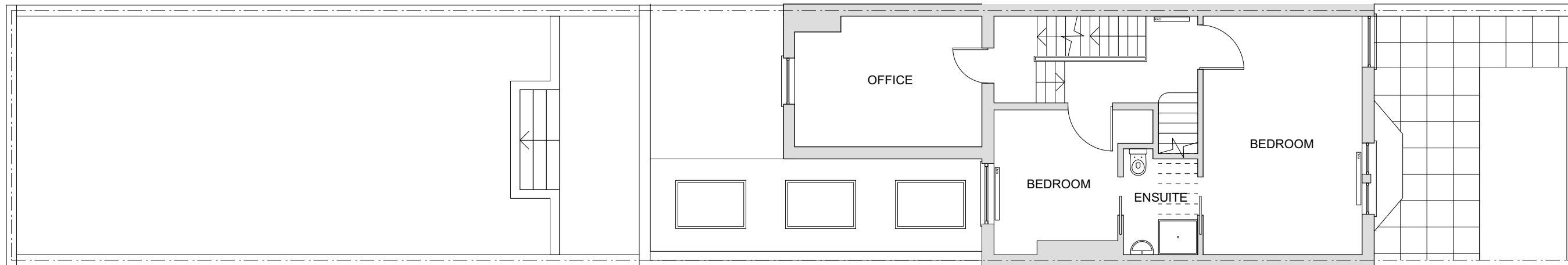
1 PROPOSED SECOND FLOOR PLAN 11
