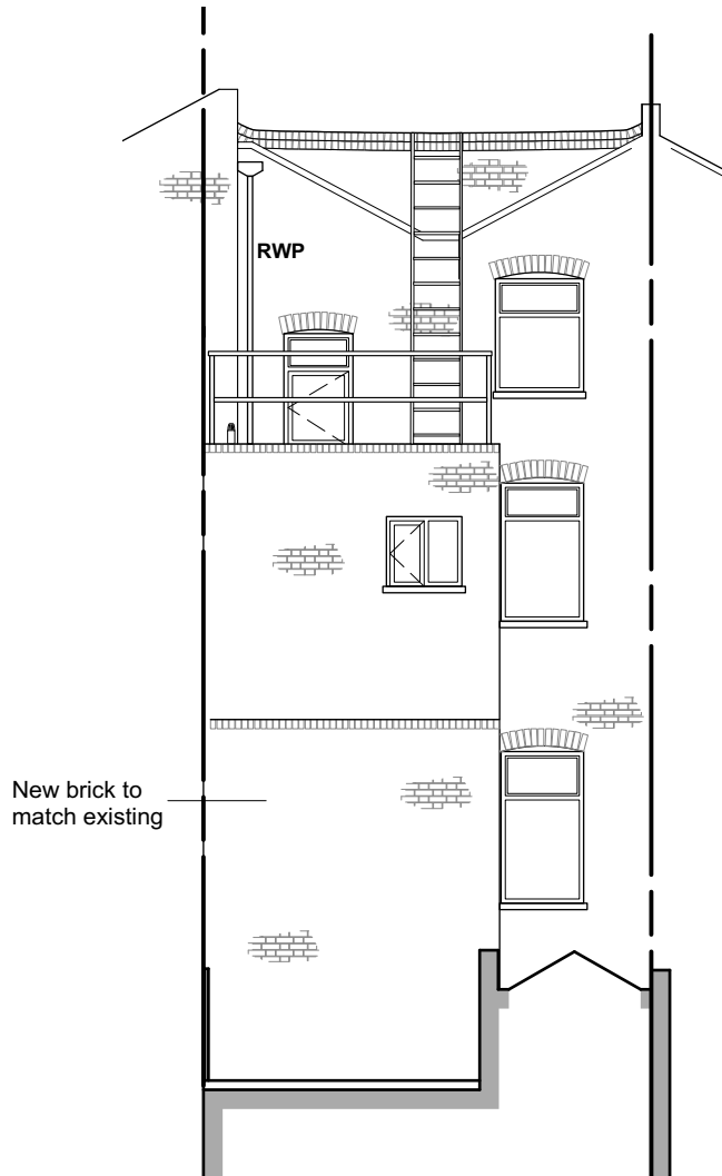
REAR ELEVATION
