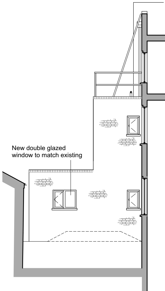
EAST ELEVATION
