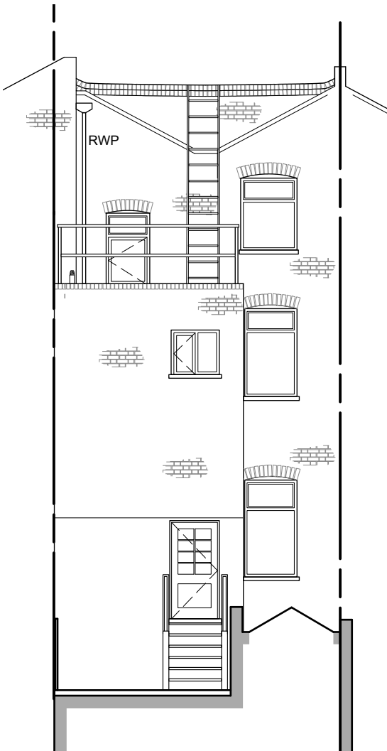
REAR ELEVATION
