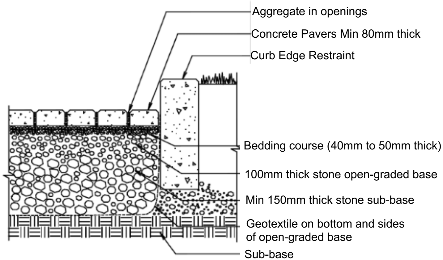
Typical Permeable Block Paving Sectional Details
