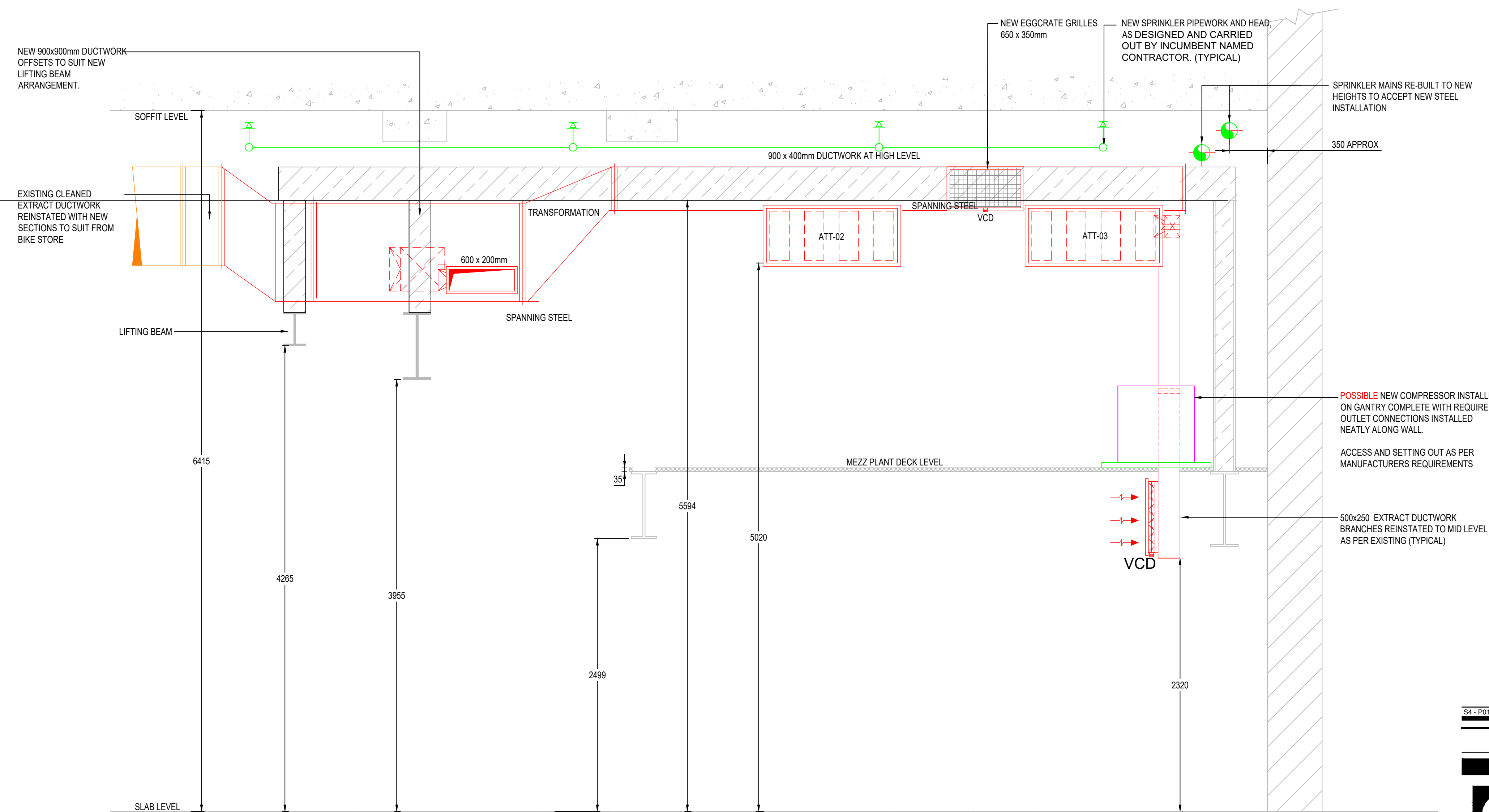
SECTION C-C
