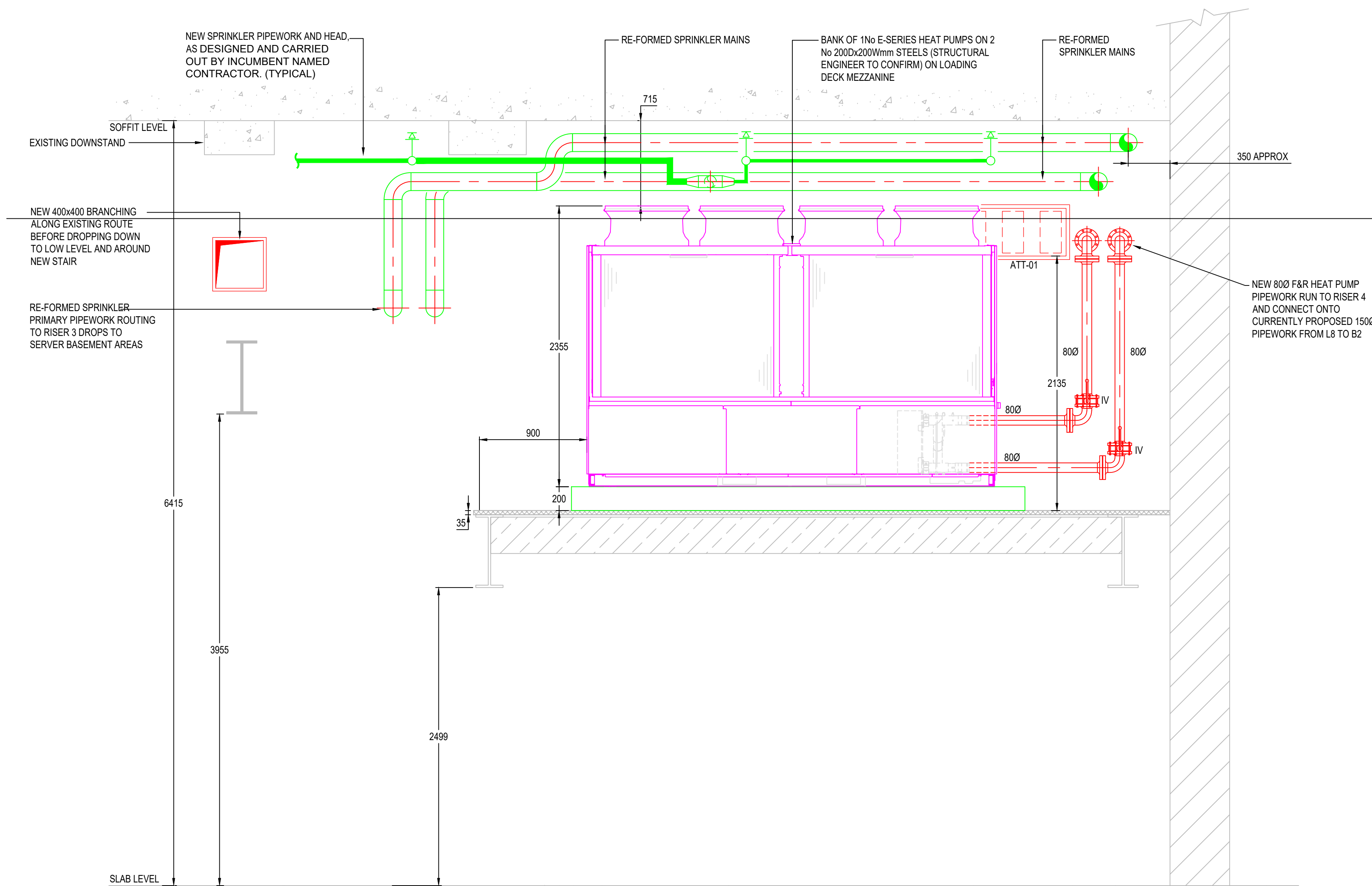
SECTION B-B H/L DUCT SECTION OMITTED FOR CLARITY
