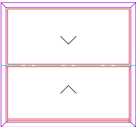
INTERNAL ELEVATION S20-VS SECONDARY GLAZING SCALE 1:20
