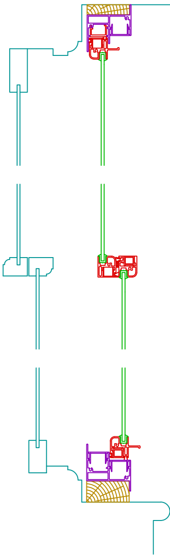
VERTICAL SECTION SCALE 1:5
