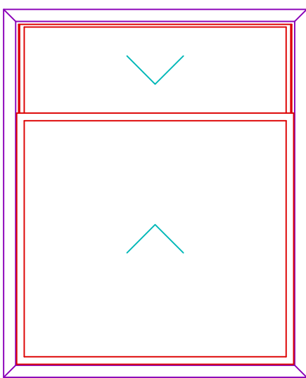
INTERNAL ELEVATION S60-TVS SECONDARY GLAZING SCALE 1:20
