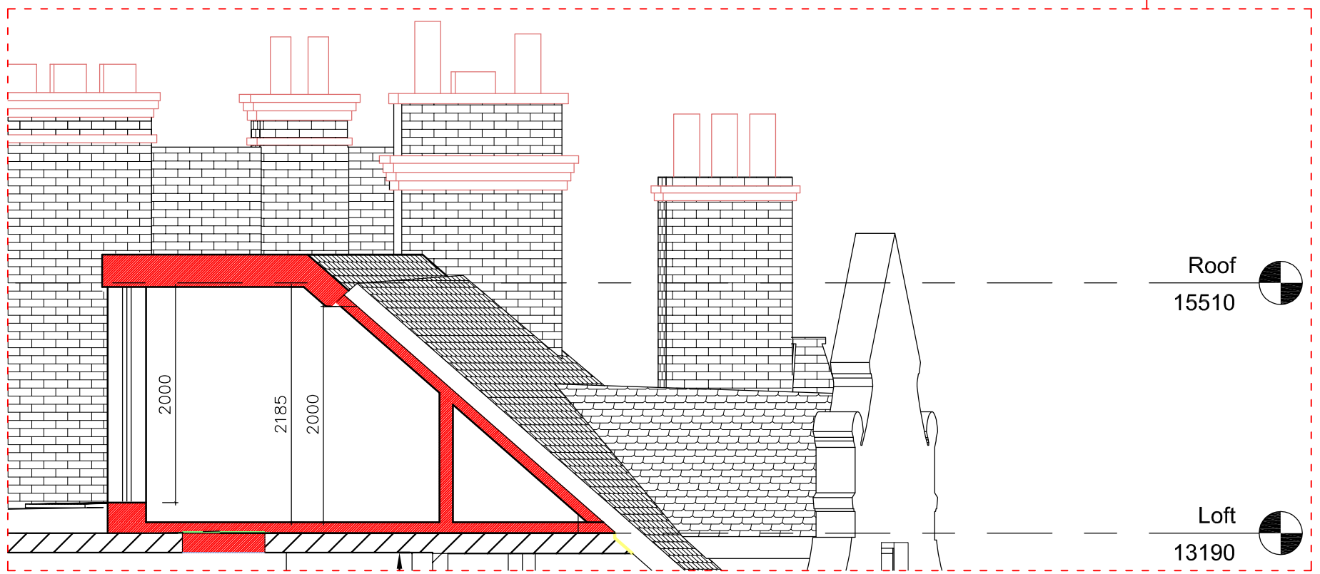
Extract of Proposed Section A-A 1:50
