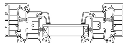
Section CC
