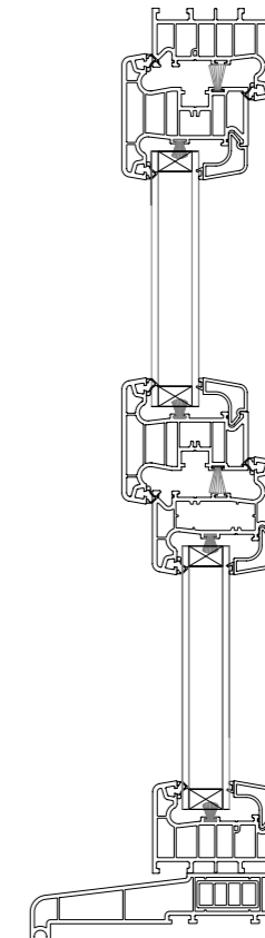
Section AA
