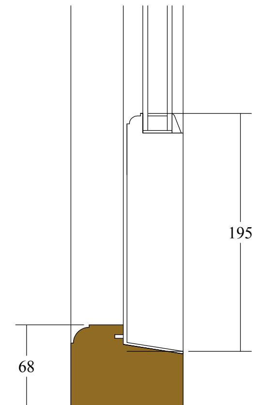
Sill Section Scale 1:3
