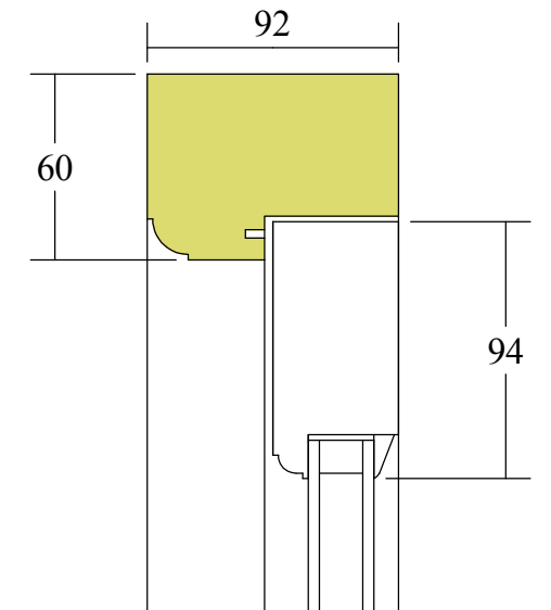
Head Section Scale 1:3
