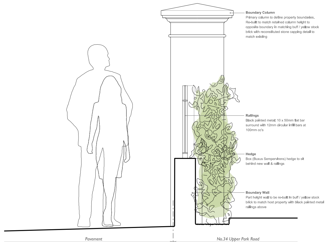
Section A - Proposed 1:20 @ A3
