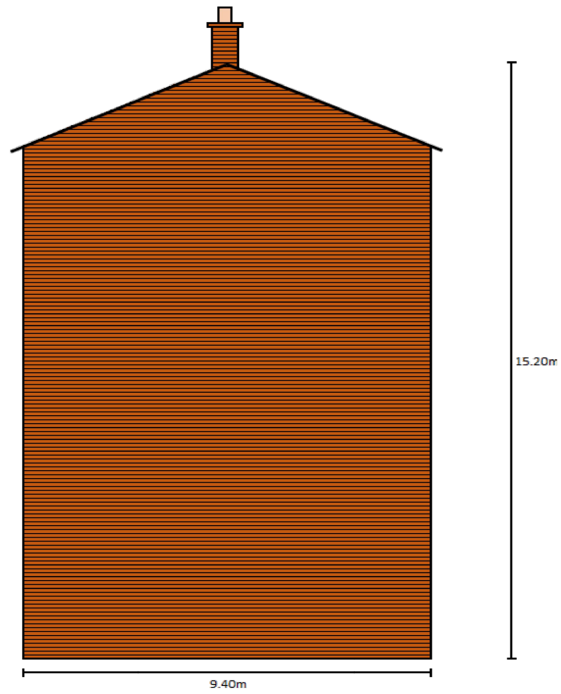
SIDE ELEVATION 01
