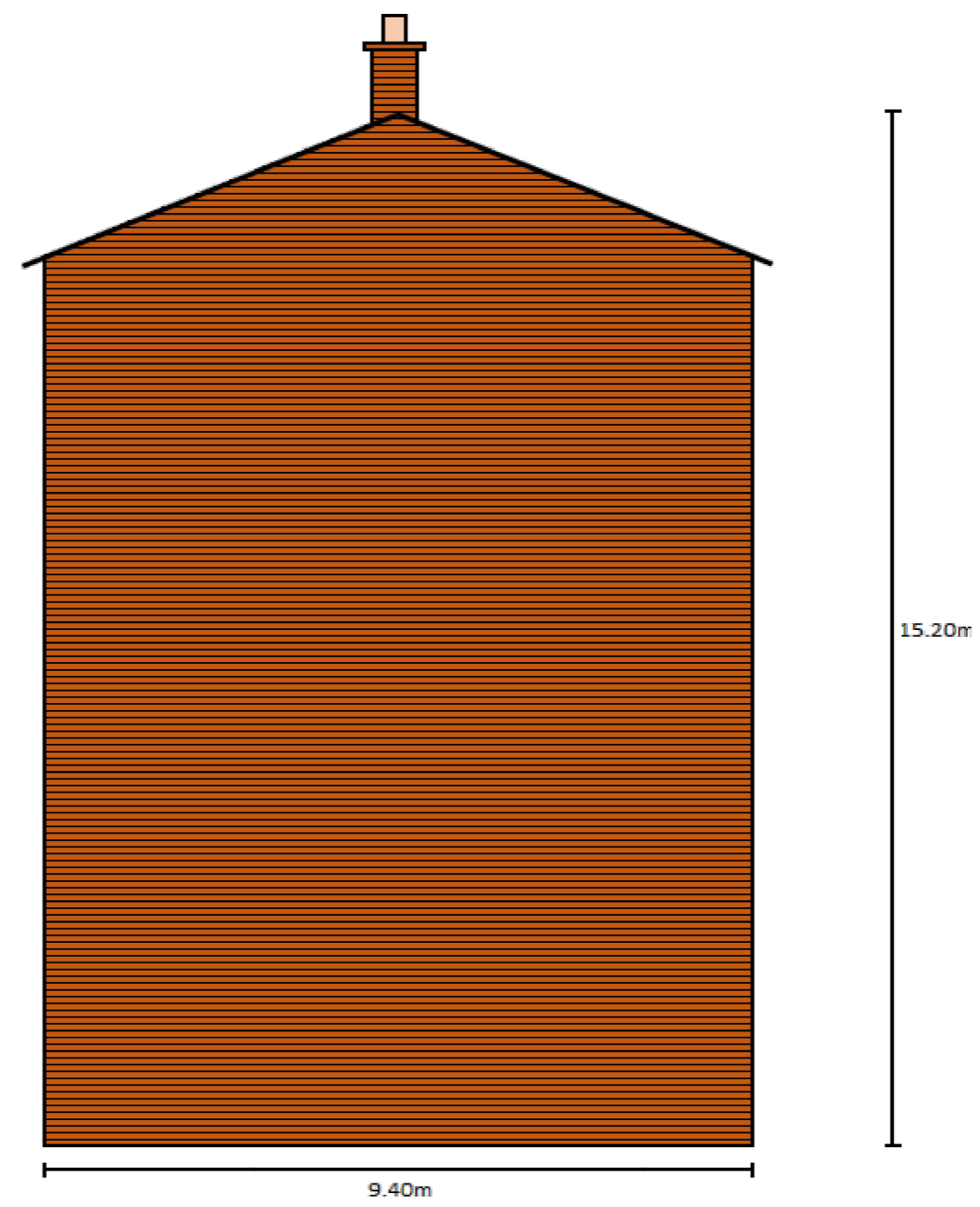
SIDE ELEVATION 02
