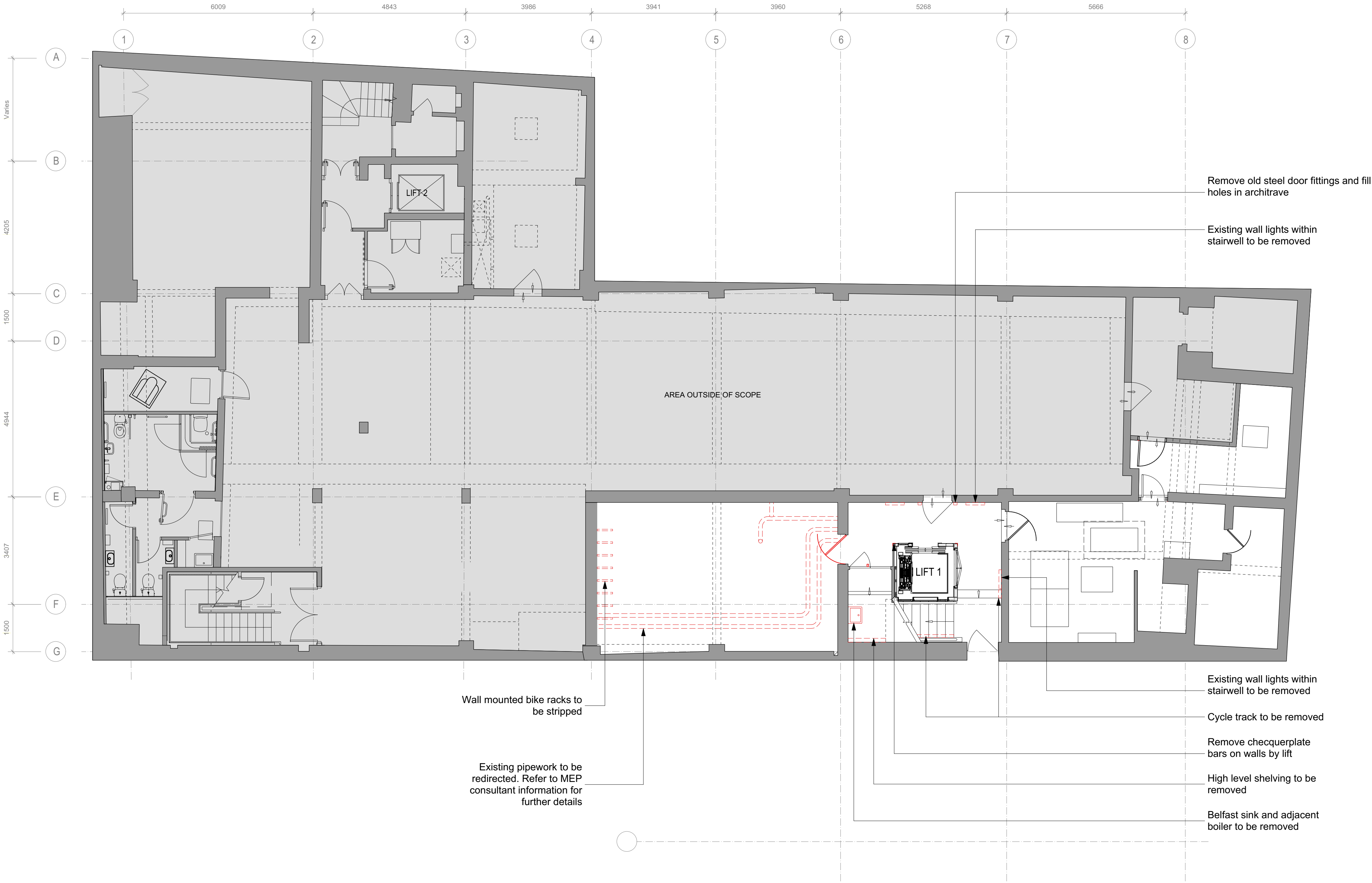
1 Basement Demolition Plan 1:75 @ A1
