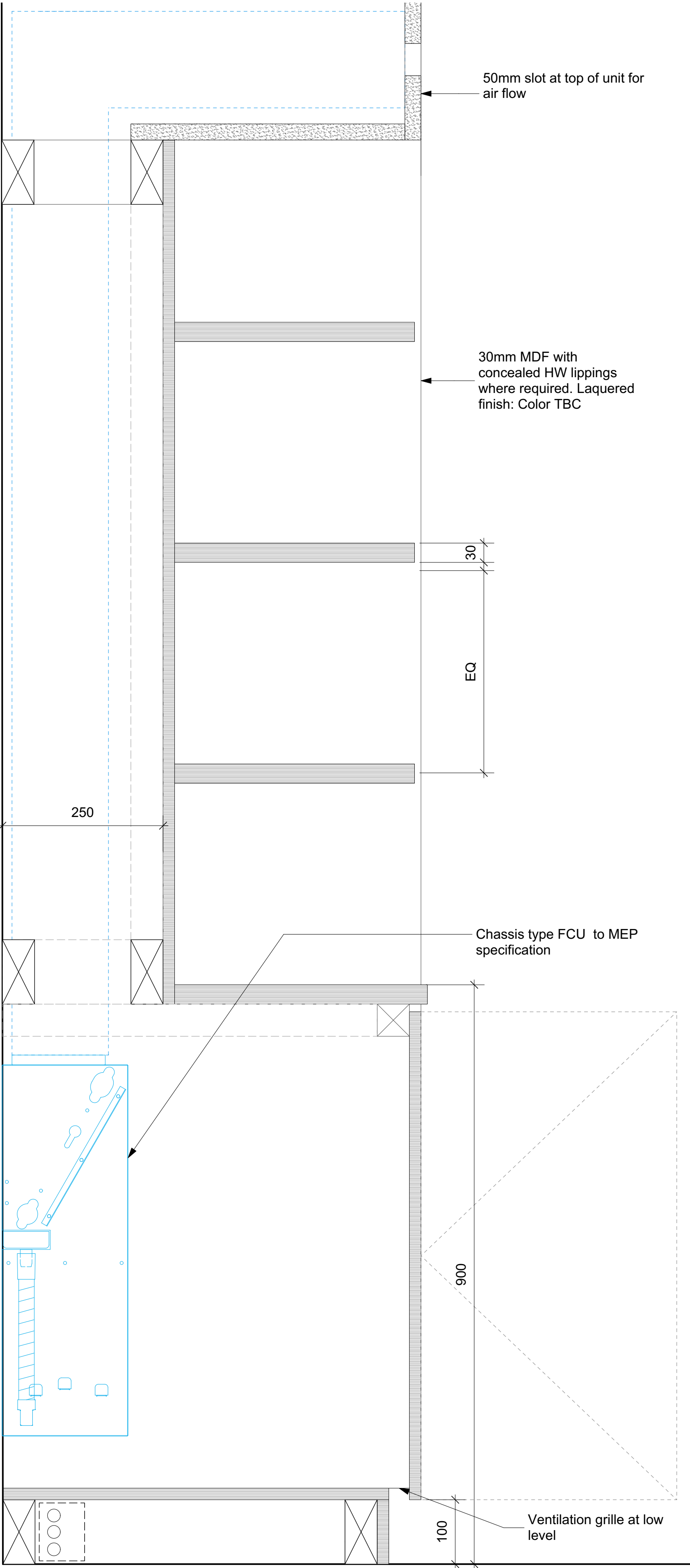
3 Fourth Floor FCU Section Scale: 1:5
