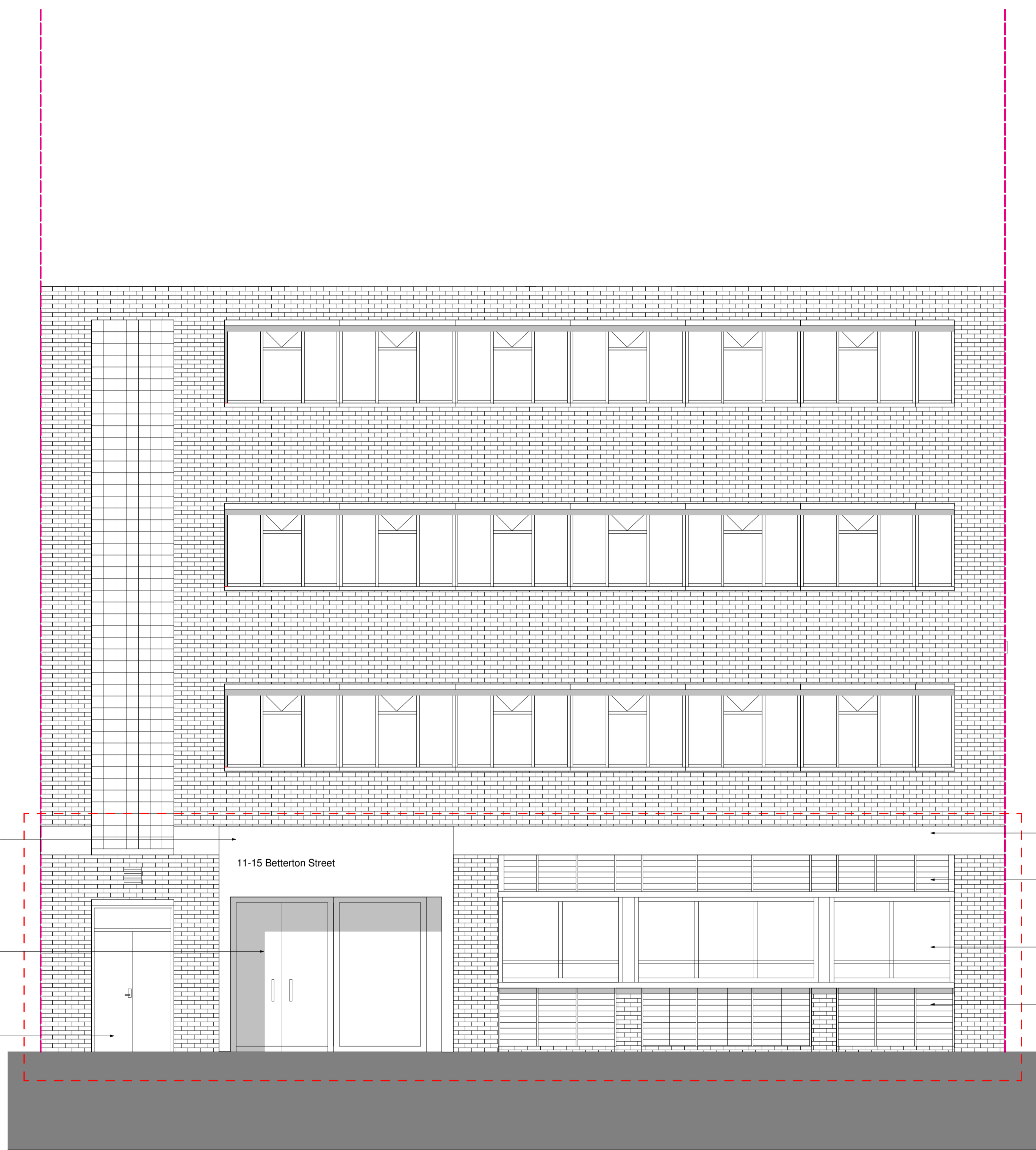
1 Betterton Street Proposed Elevation 1 (ROLLER SHUTTER OPEN) Scale 1 : 50
