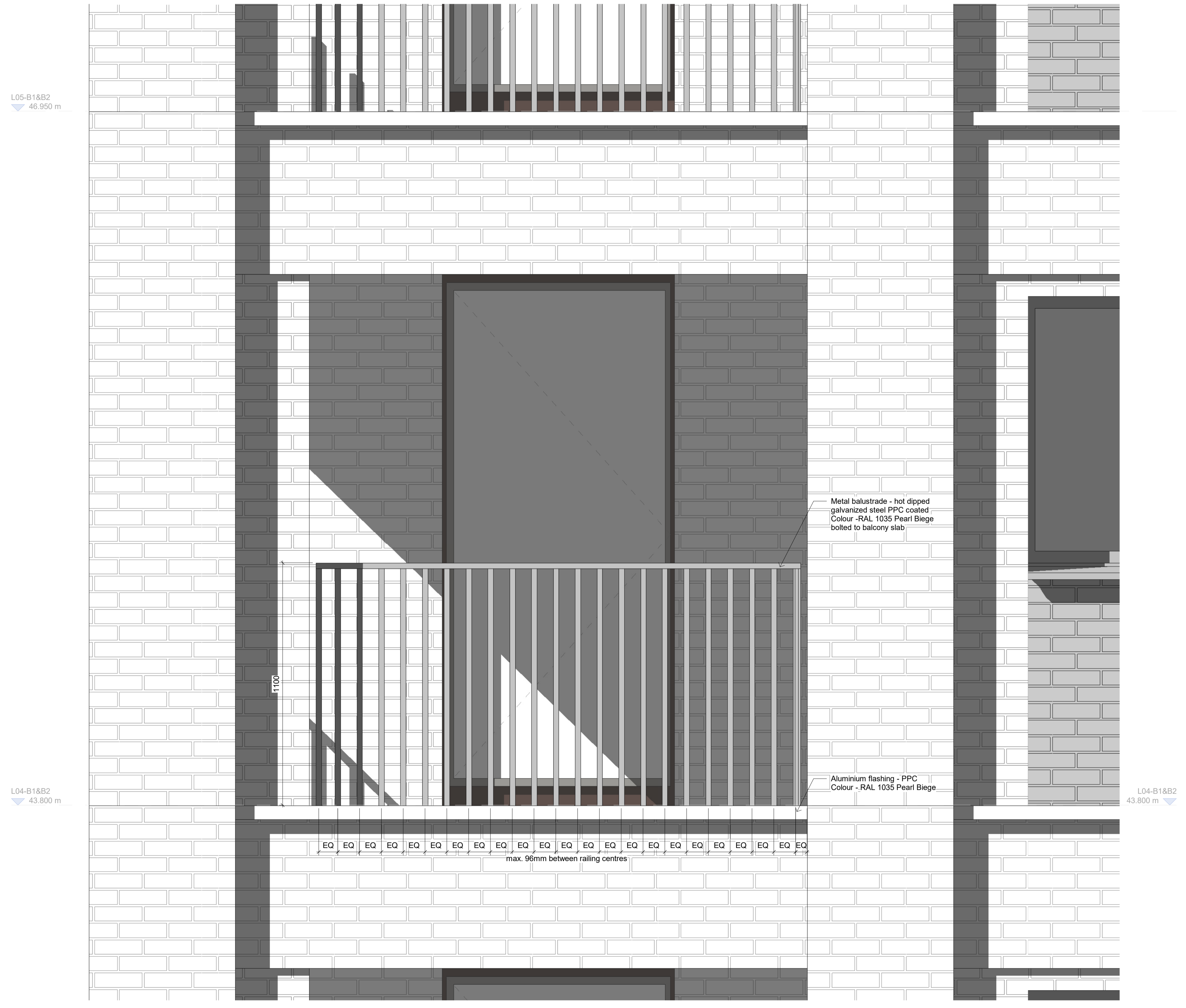
1 Typical balcony balustrade elevation 1:10
