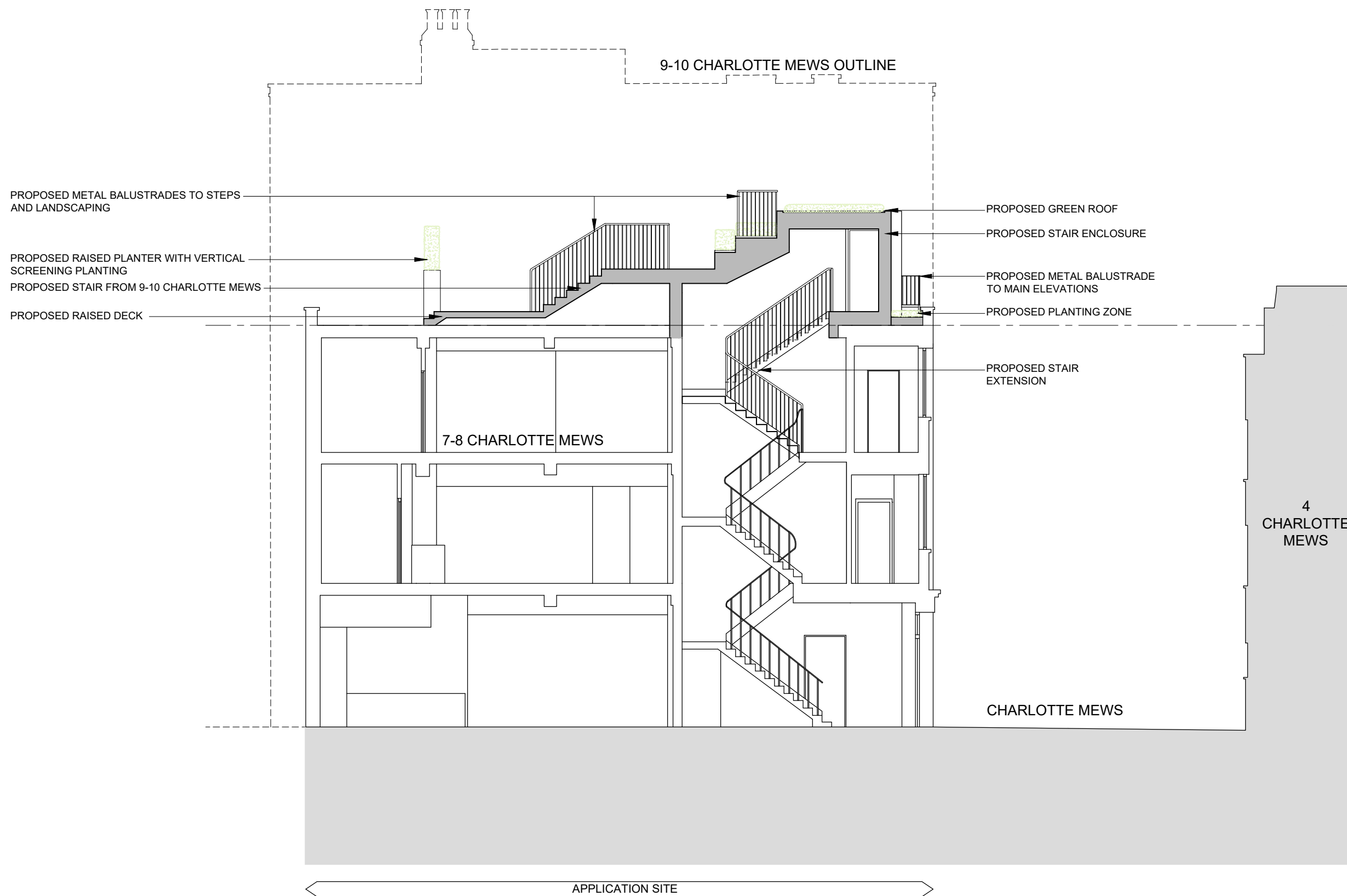
AA - CROSS SECTION
