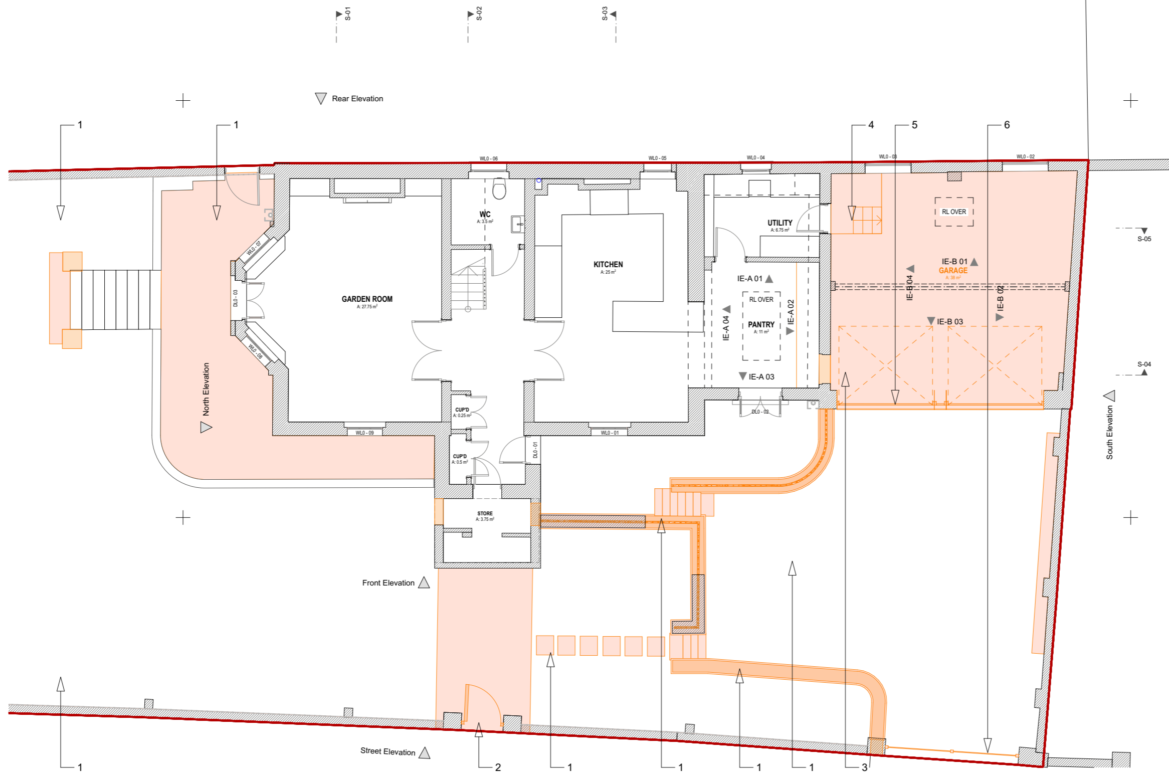
-1. Lower Ground Floor 1:100
