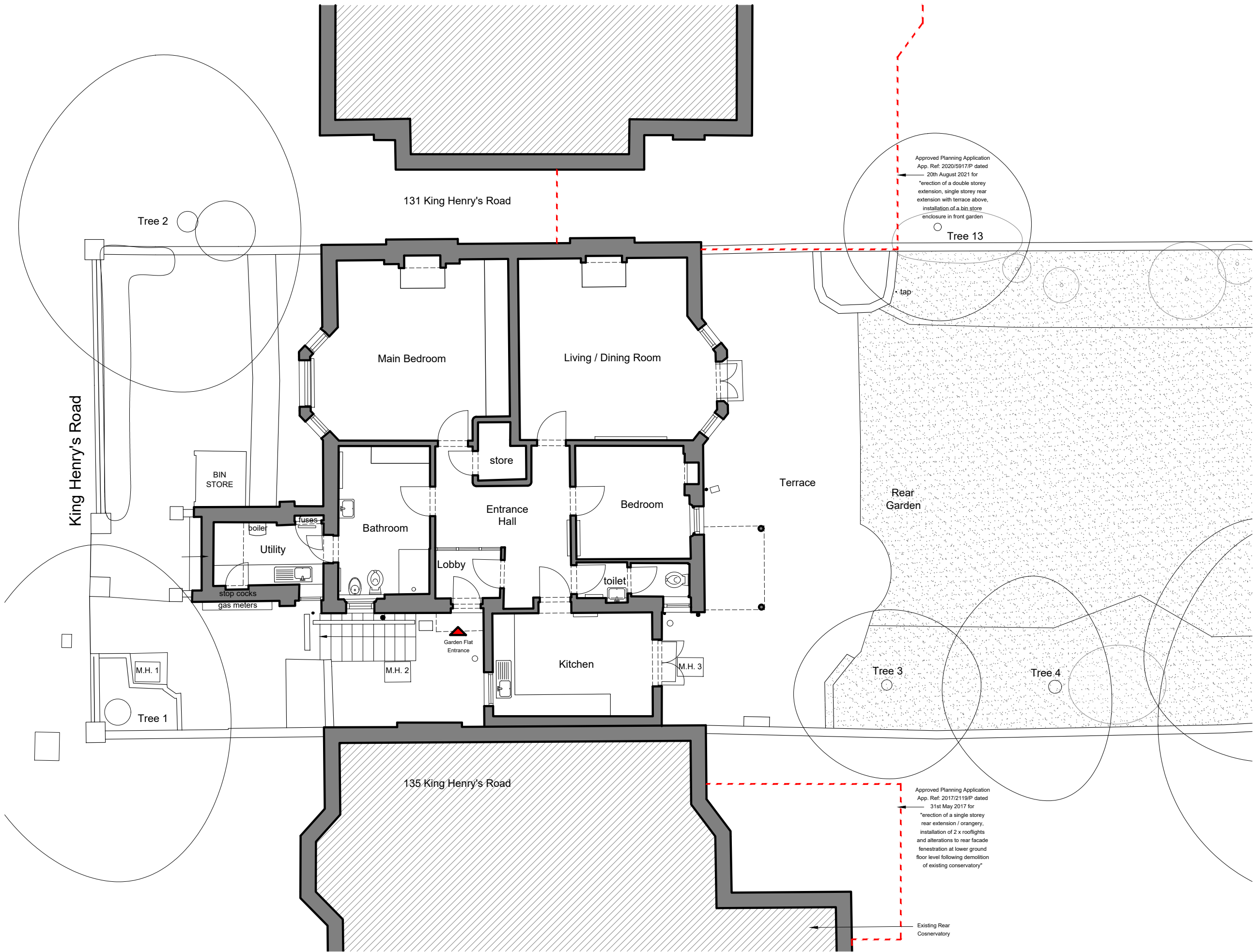
EXISTING - Garden Flat Floor Plan Scale 1:100@A3 EX-01
