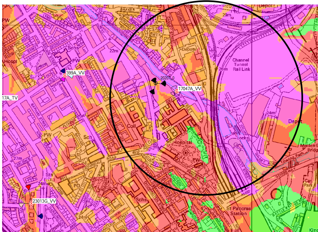
Fig. 3: Proposed LTE2100 coverage (replacement 20207)
