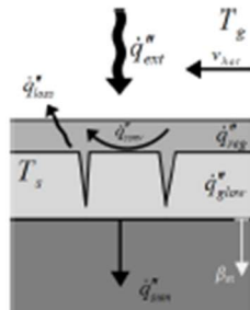
Figure 5: Heat transfer elements contributing to superimposed heat flux \dot{q}_{sum} relevant for the charring rate \beta_{st} .
