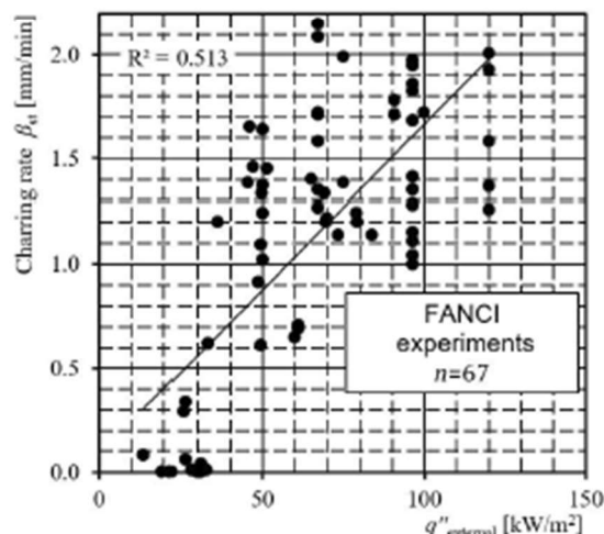
Figure 7: Observed charring rate vs. external heat flux and the correlation coefficient (least squares method).
