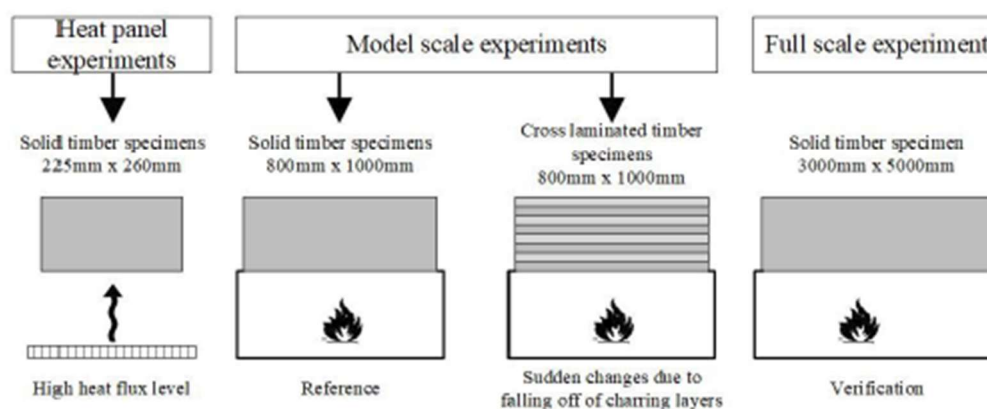
Figure 3: Experimental setups performed in the presented campaign.
