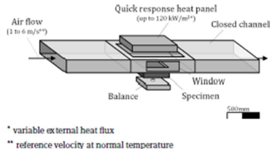
Figure 6: The Fire Apparatus for Non-standard heating and Charring Investigation (FANCI).
