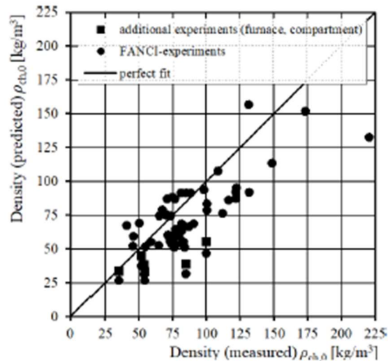
Figure 10: Measured vs. predicted char layer density.
