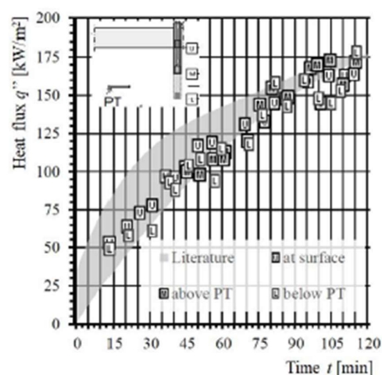
Figure 4: Measurements of the HFS at the positions "Upper" "Medium" and "Lower" in comparison to results available in the literature [14].
