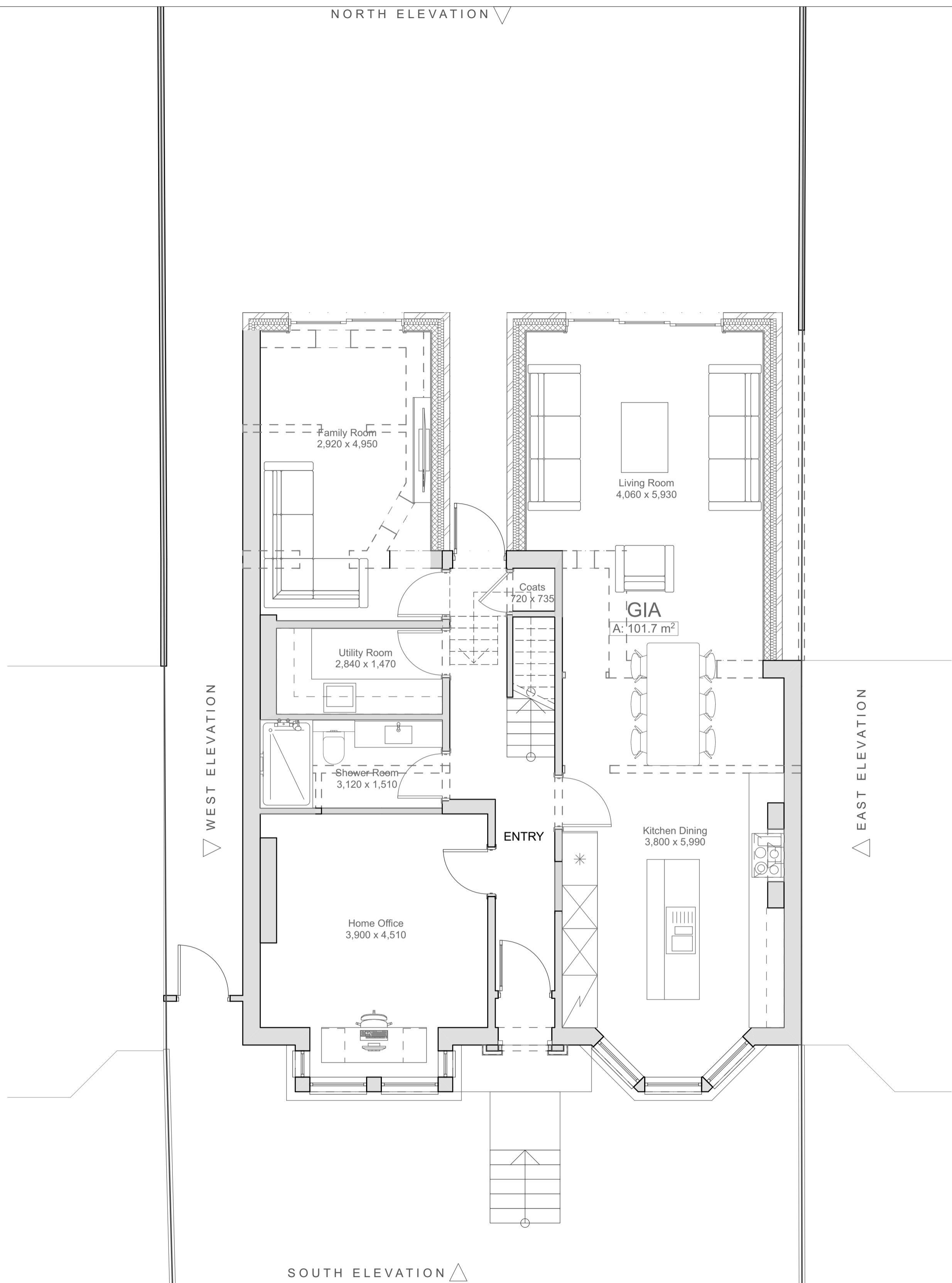
APPROVED GROUND 1:50
