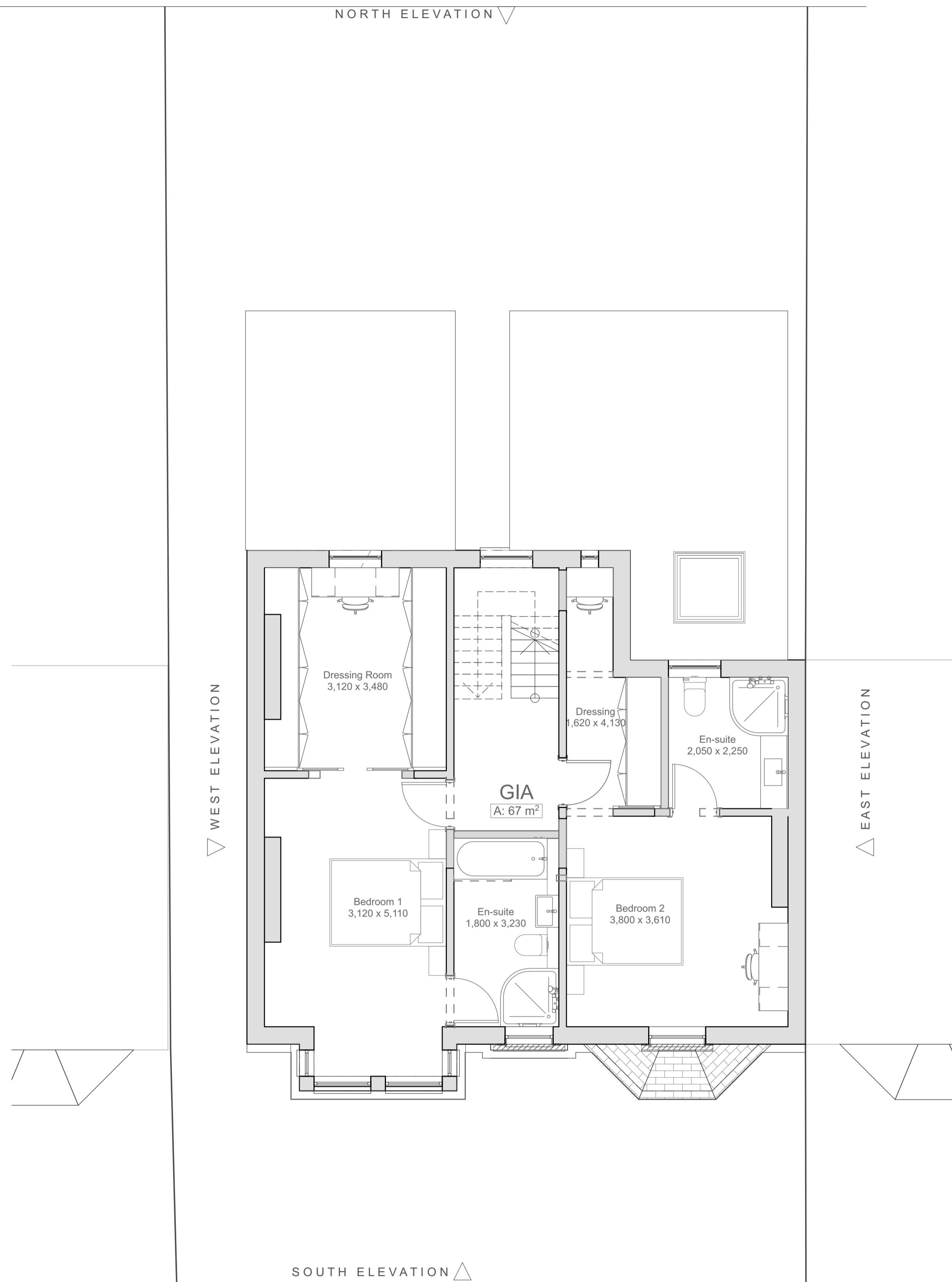
APPROVED FIRST 1:50
