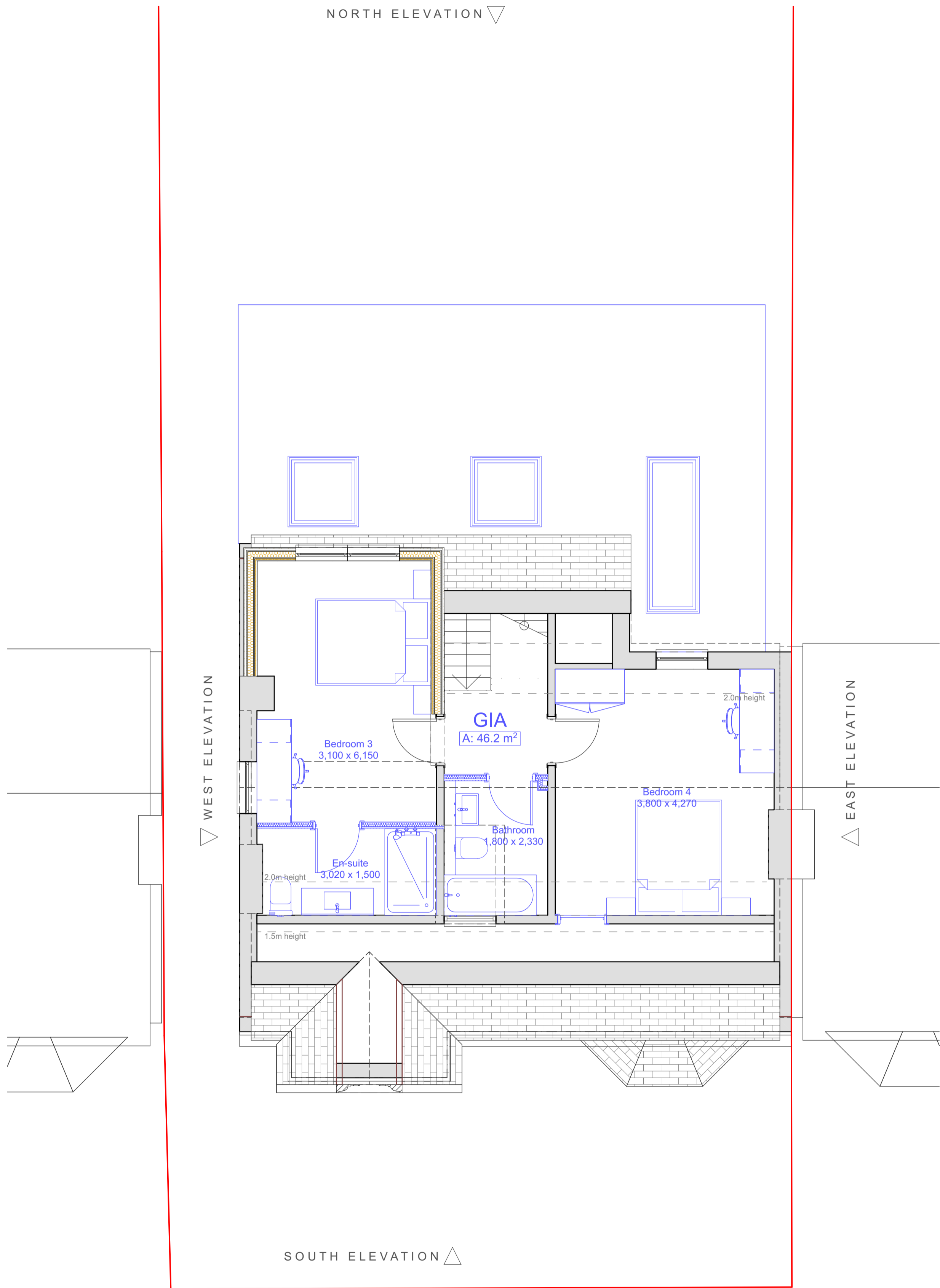
PROPOSED ATTIC 1:50
