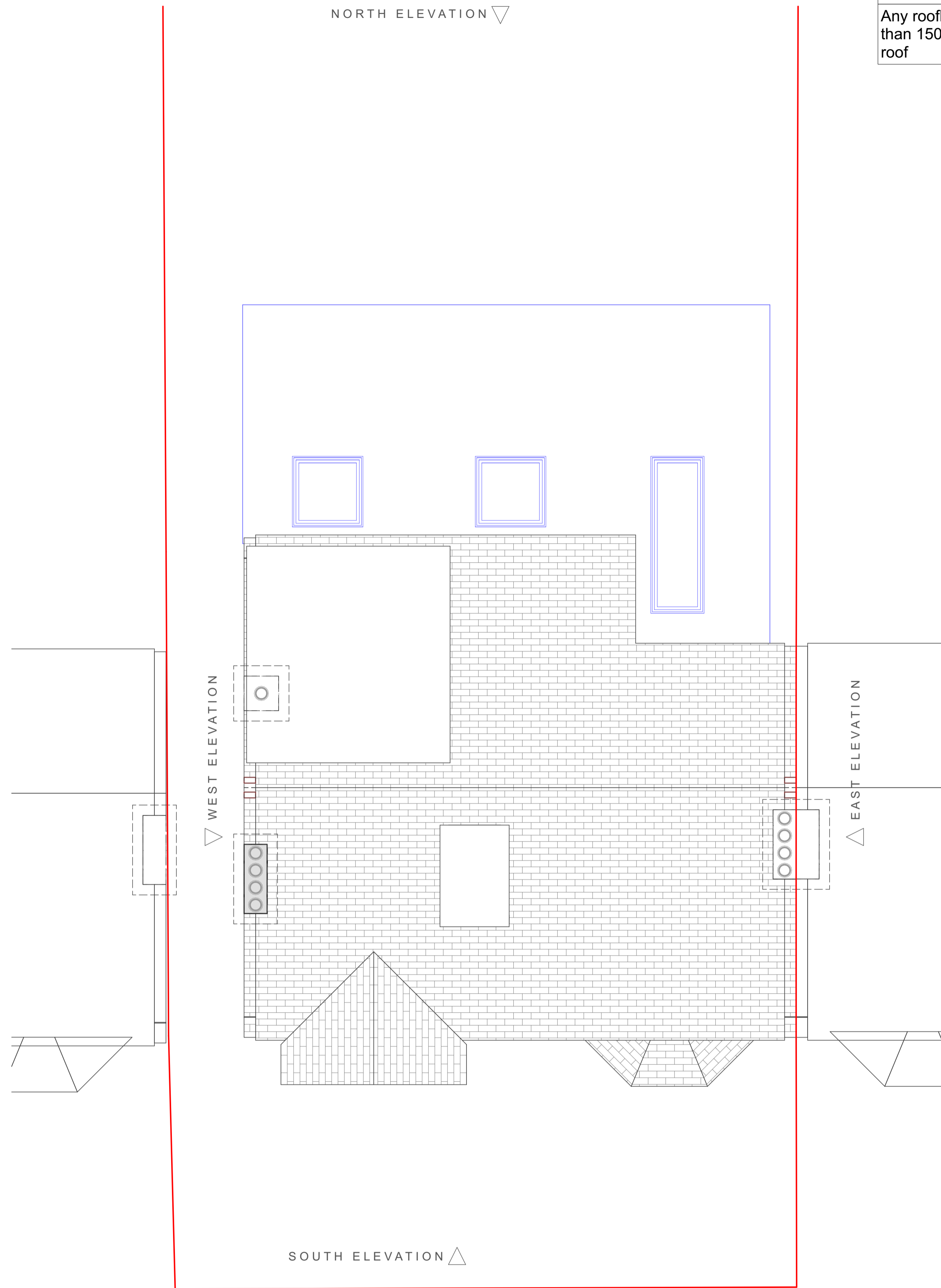
PROPOSED ROOF 1:50
