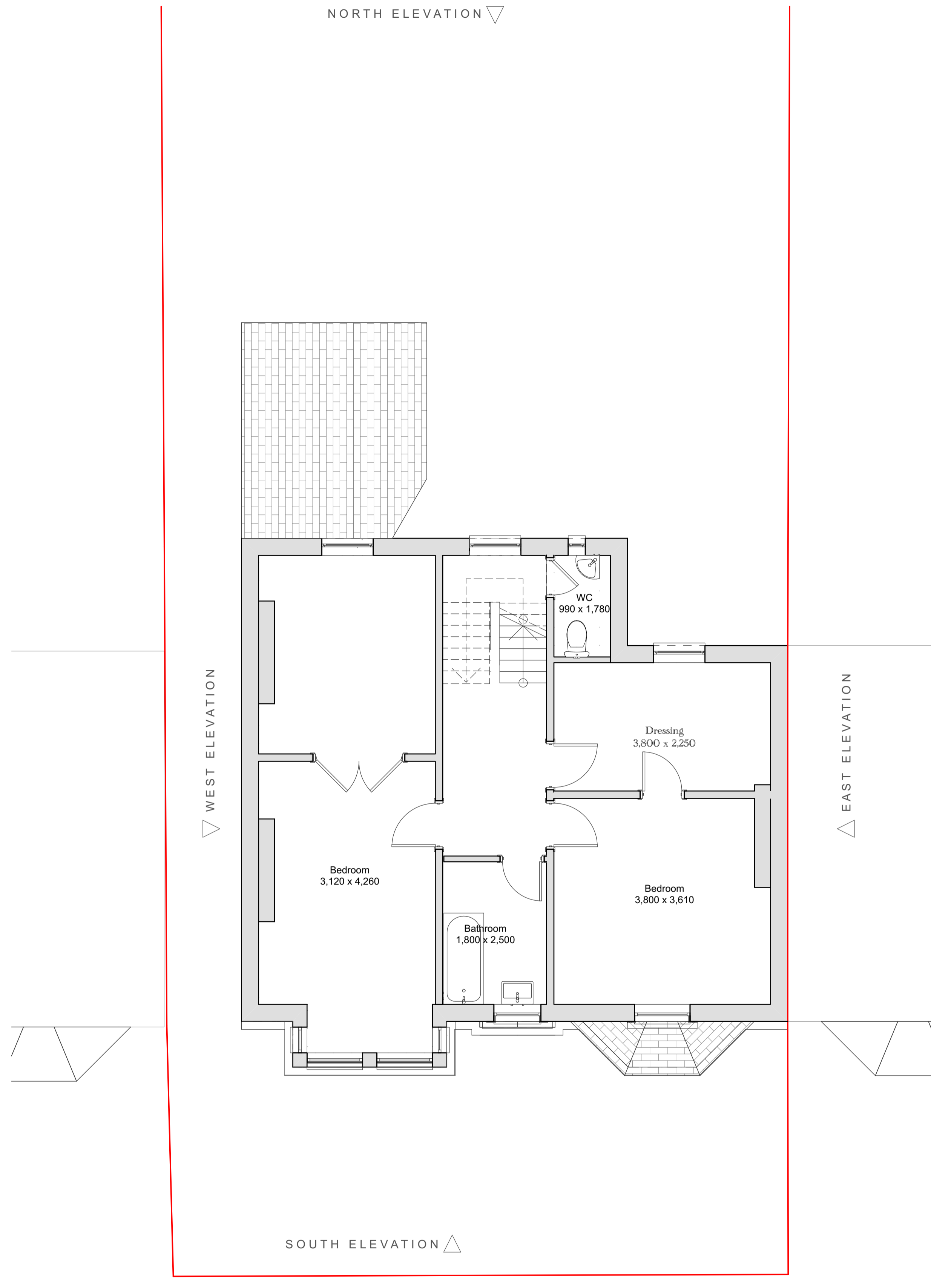
EXISTING FIRST 1:50
