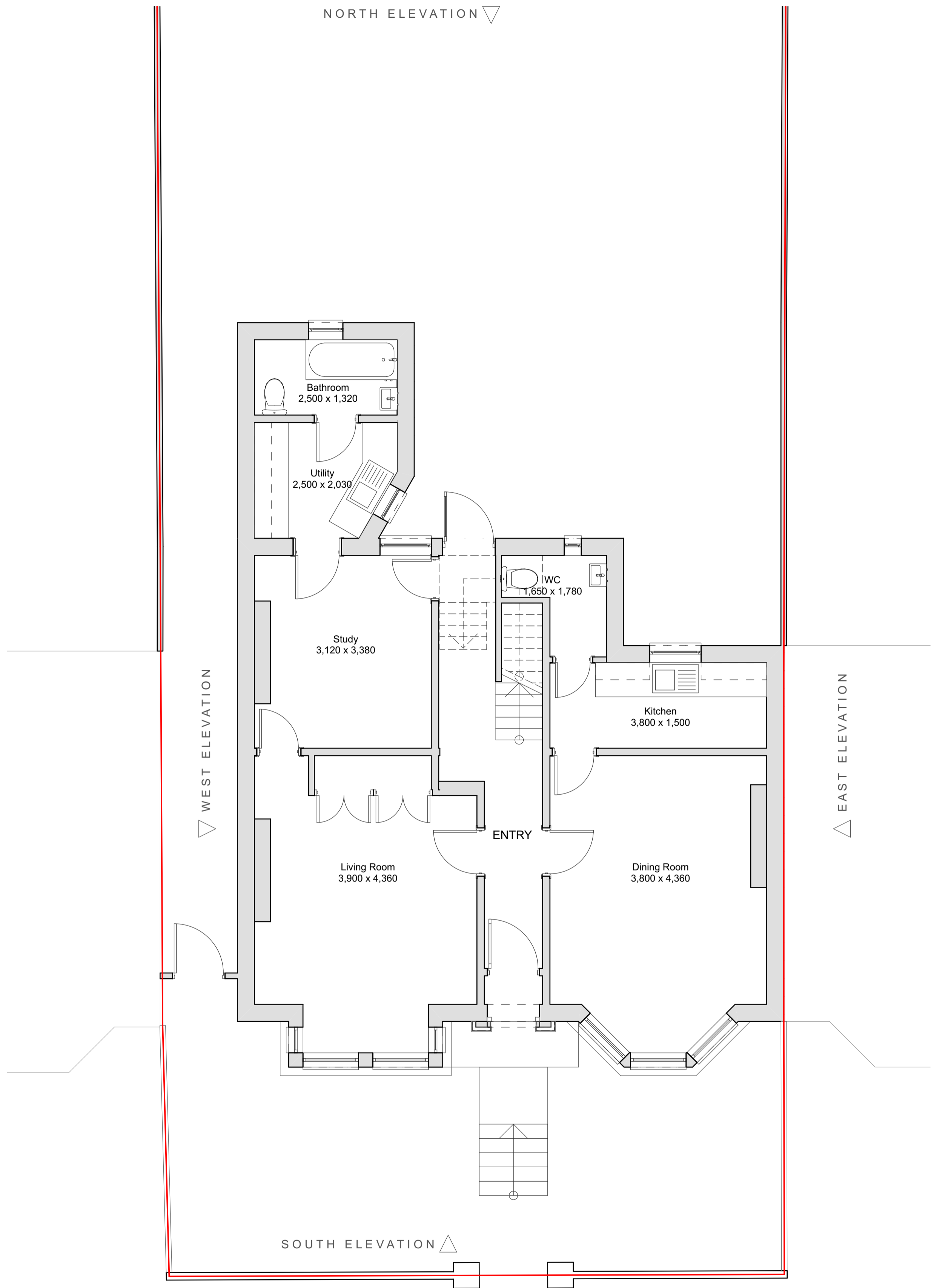
EXISTING GROUND 1:50
