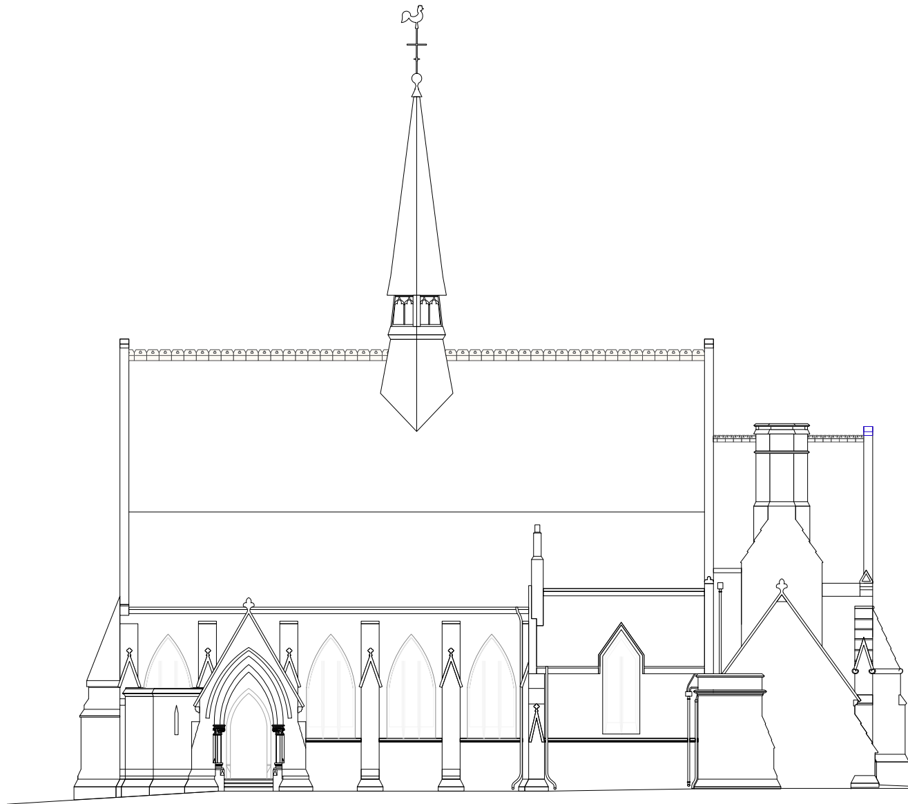
South Elevation
