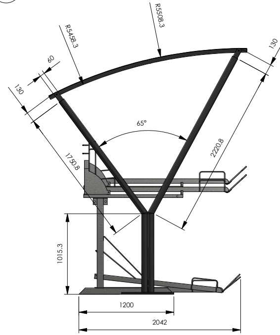
SIDE ELEVATION
