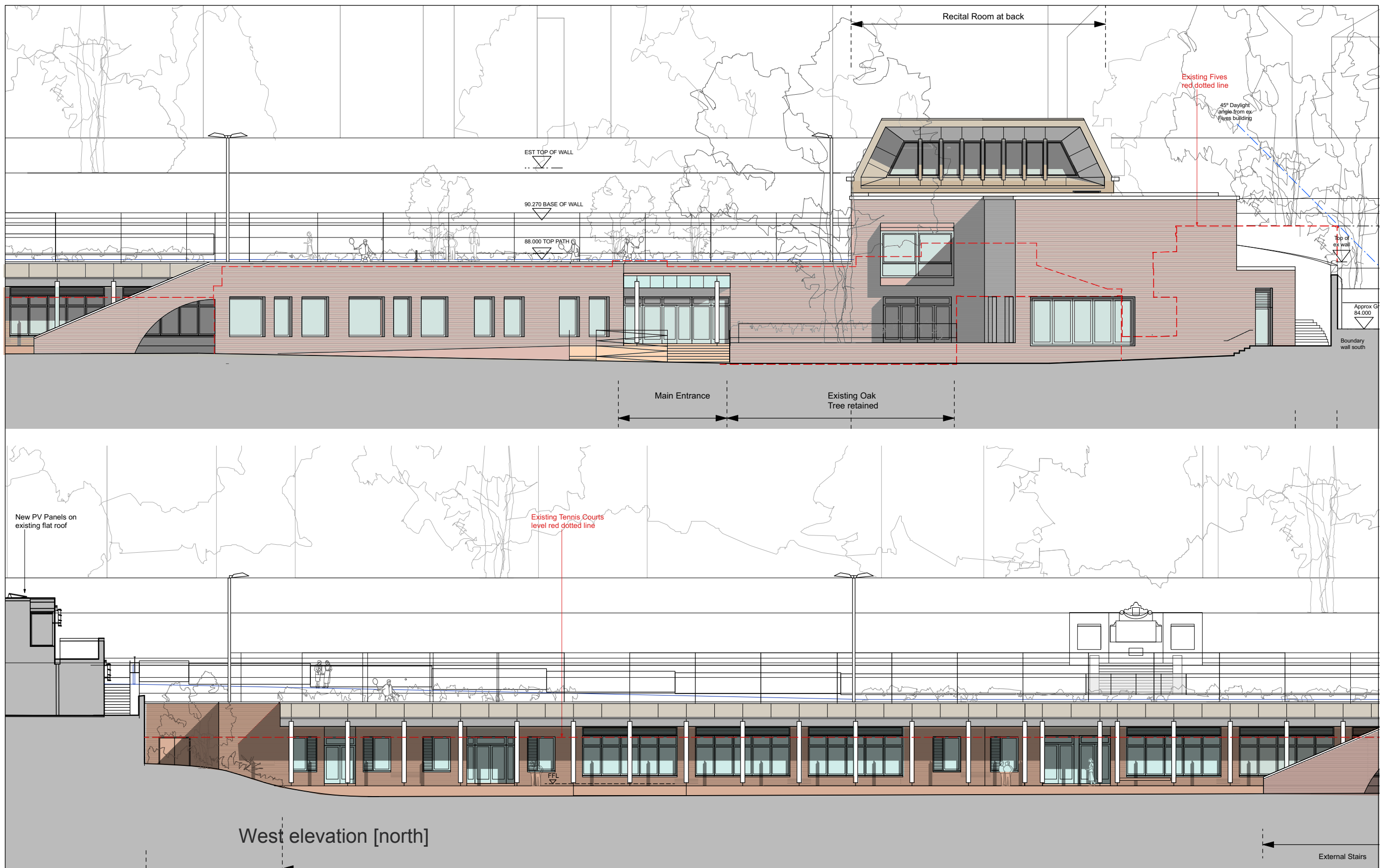
Part Detail West elevation South [top] and North [bottom]
