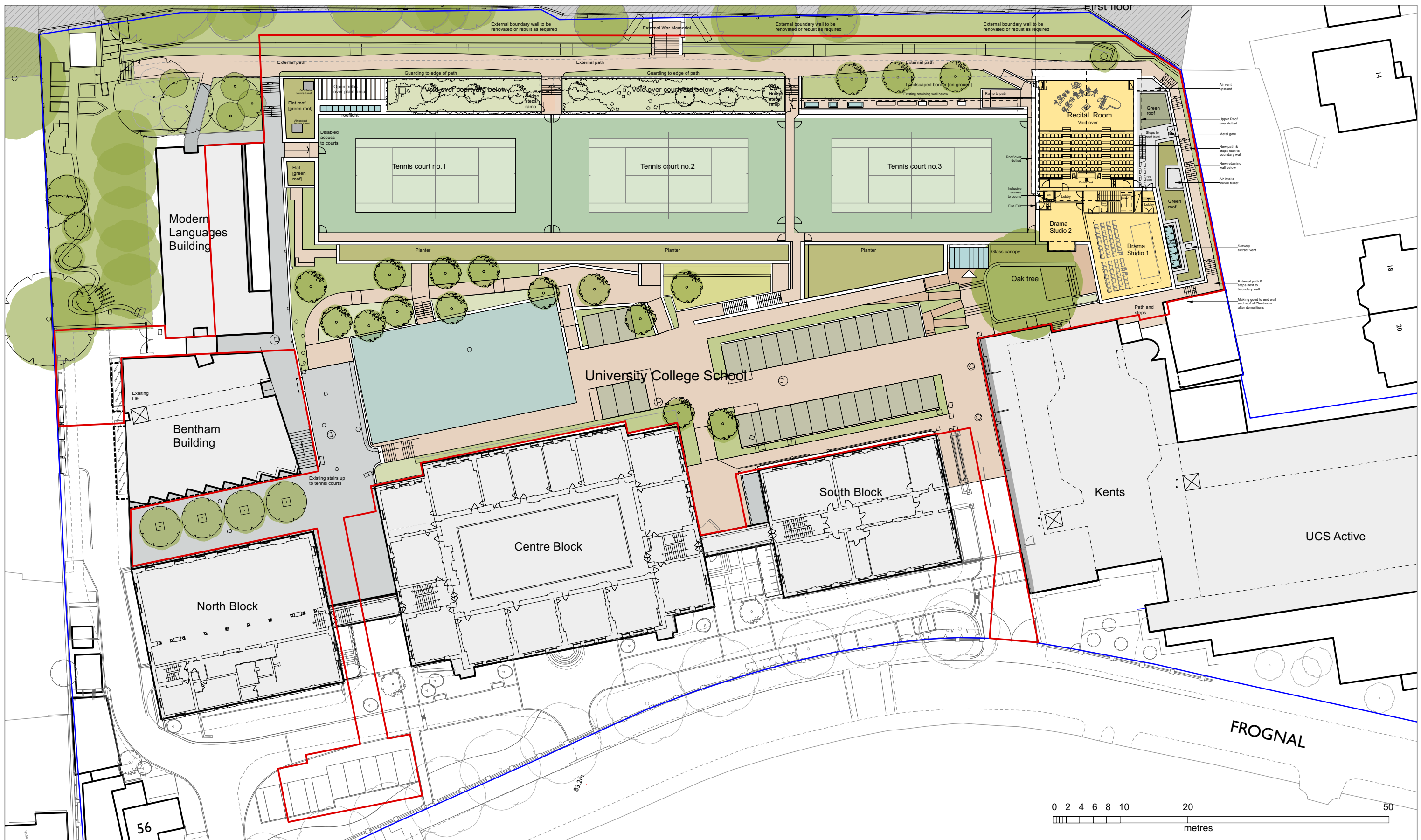
First floor plan in garden landscape setting, with tennis courts, rooftop planters, green roofs
