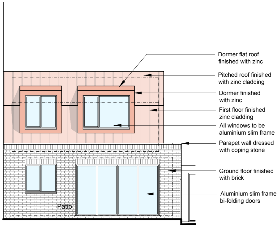
New Building - Rear Elevation As Proposed 1:100
