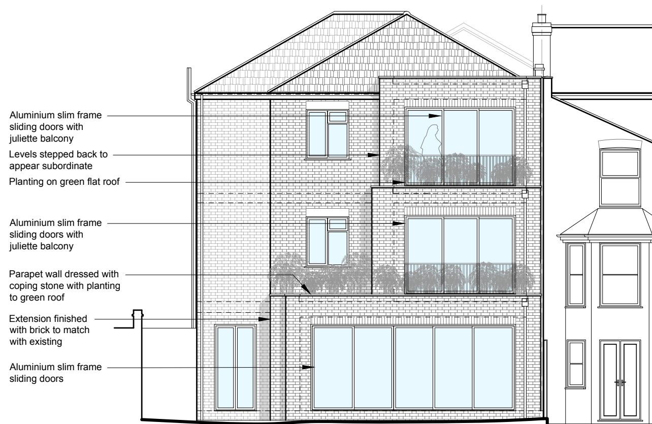
Flats - Rear Elevation As Proposed 1:100
