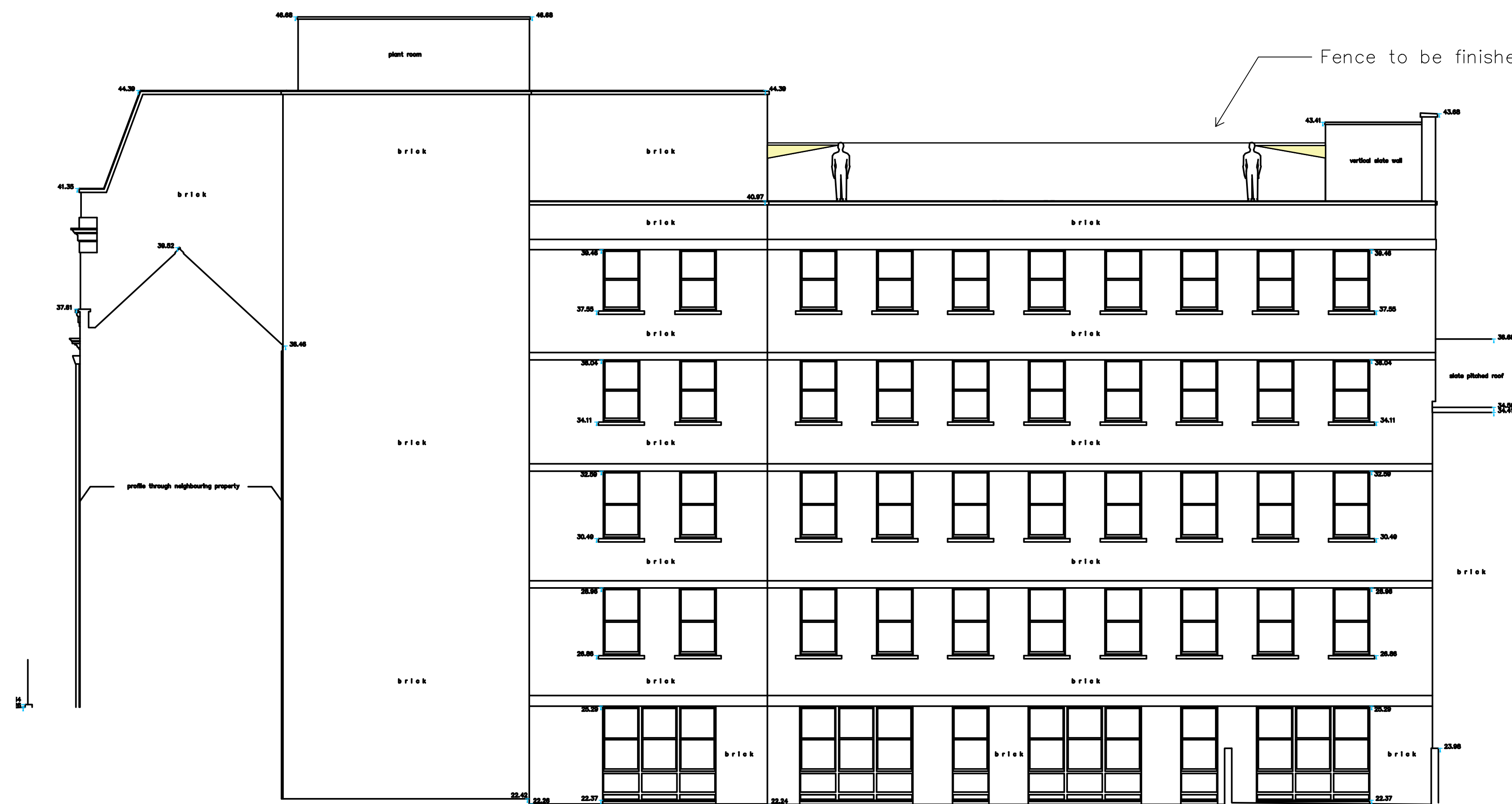
Section CC
