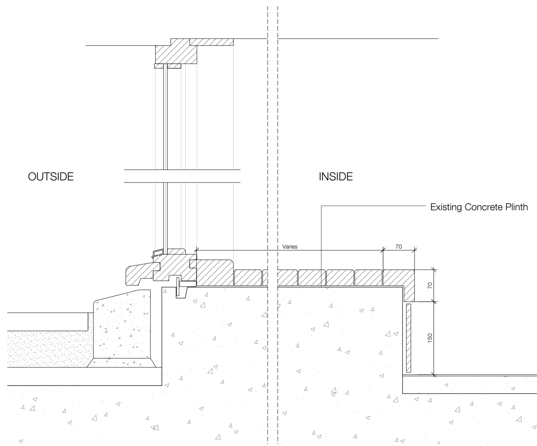
01 Block A - Plinth Details 1.5
