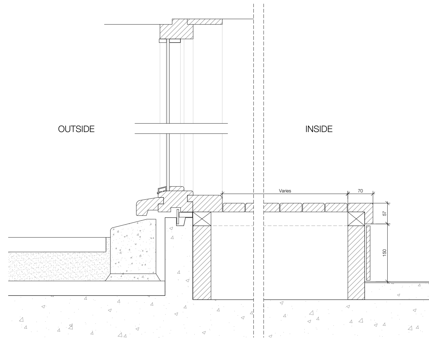
02 Block B - Plinth Details 1.5
