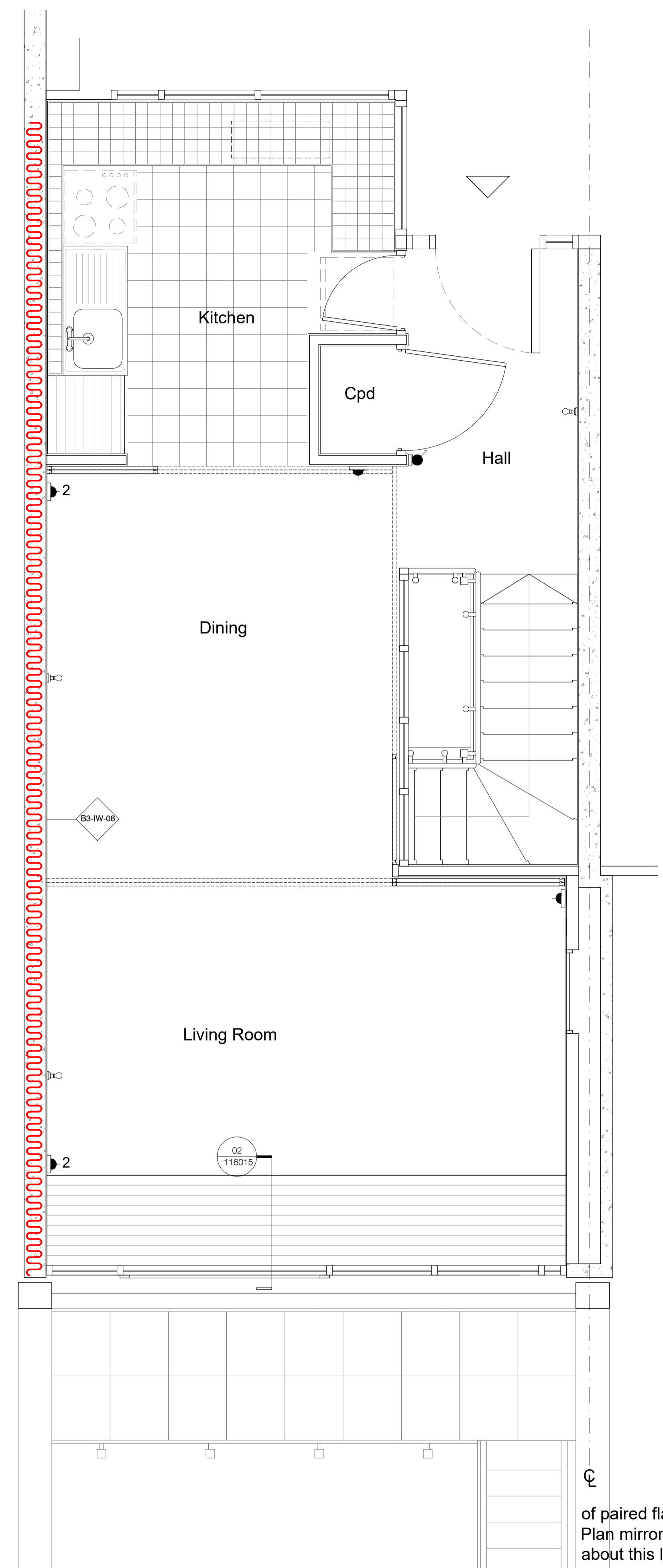
02 Dwelling Type B3 - Upper Level Plan 1:25
