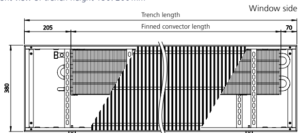
Top view of trench height 150/200 mm (view without cover panel)
