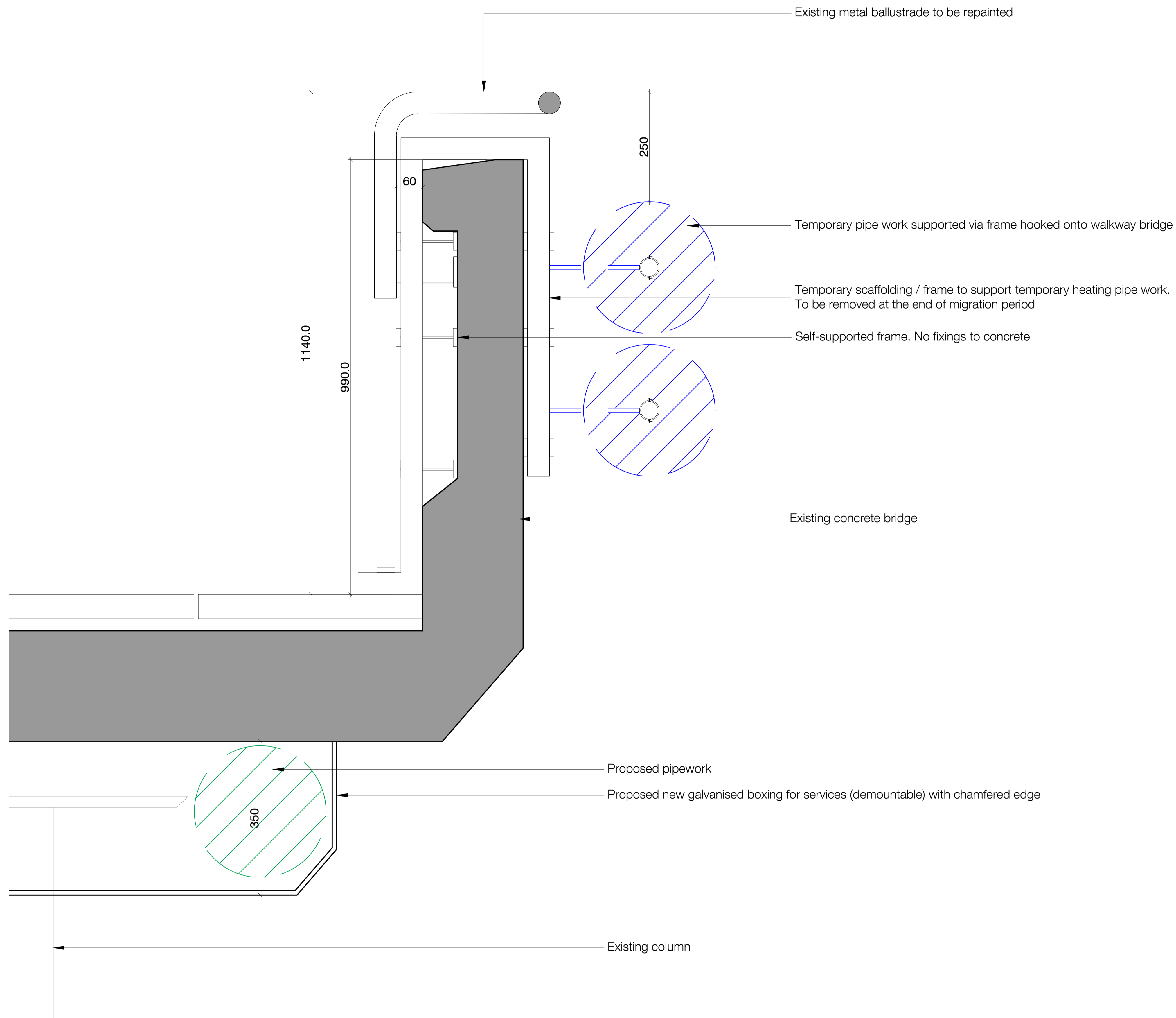
01 Detail - Temporary support frame for heating pipe work in Bridge 331004
