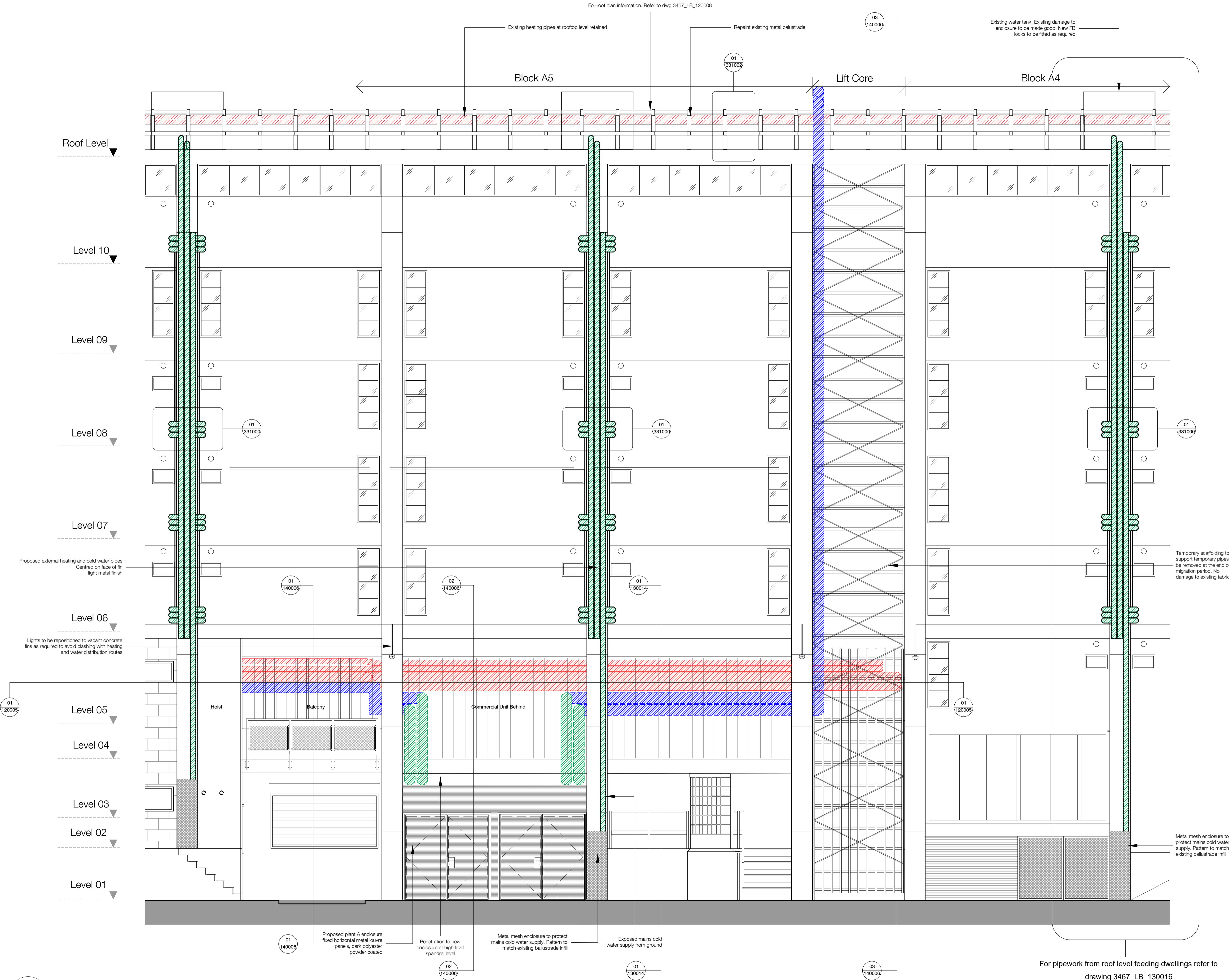
01 Block A - Existing and Temporary - Distribution Route from Housing Office Balcony to Roof - Elevation 1:50
