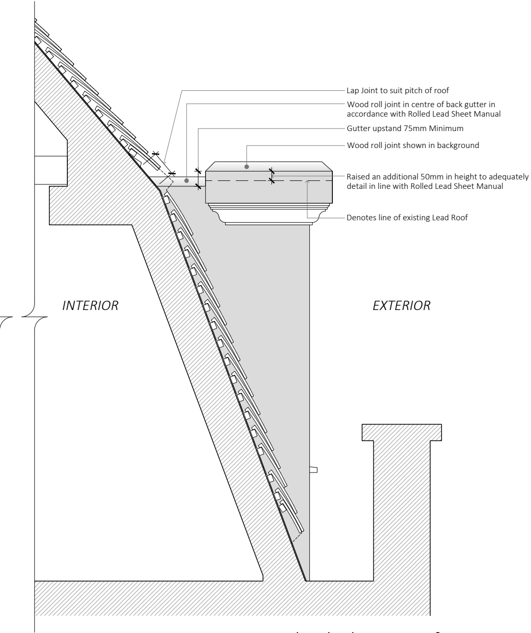
Dormer Cheek Elevation of New Proposed Lead Roof
