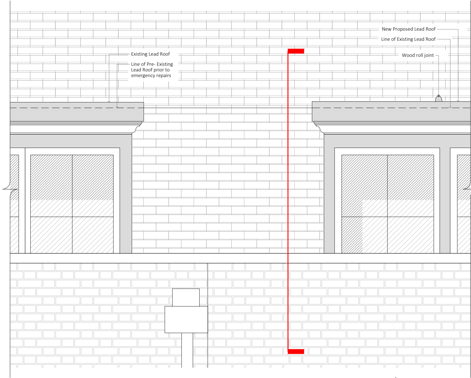
Part Dormer Elevation
