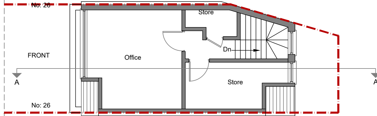
THIRD FLOOR PLAN ( No proposed changes to Floor Plan)
