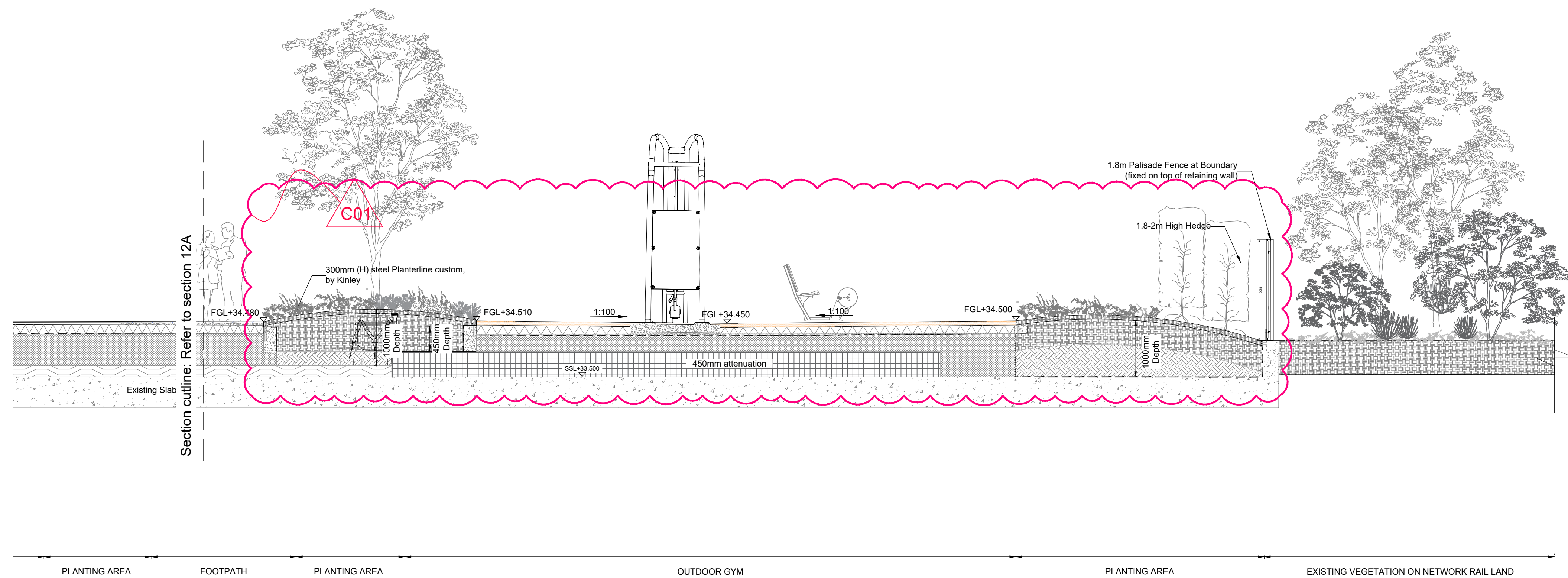
12B Stairs (Mid Point) to Railway Park Scale: 1:50
