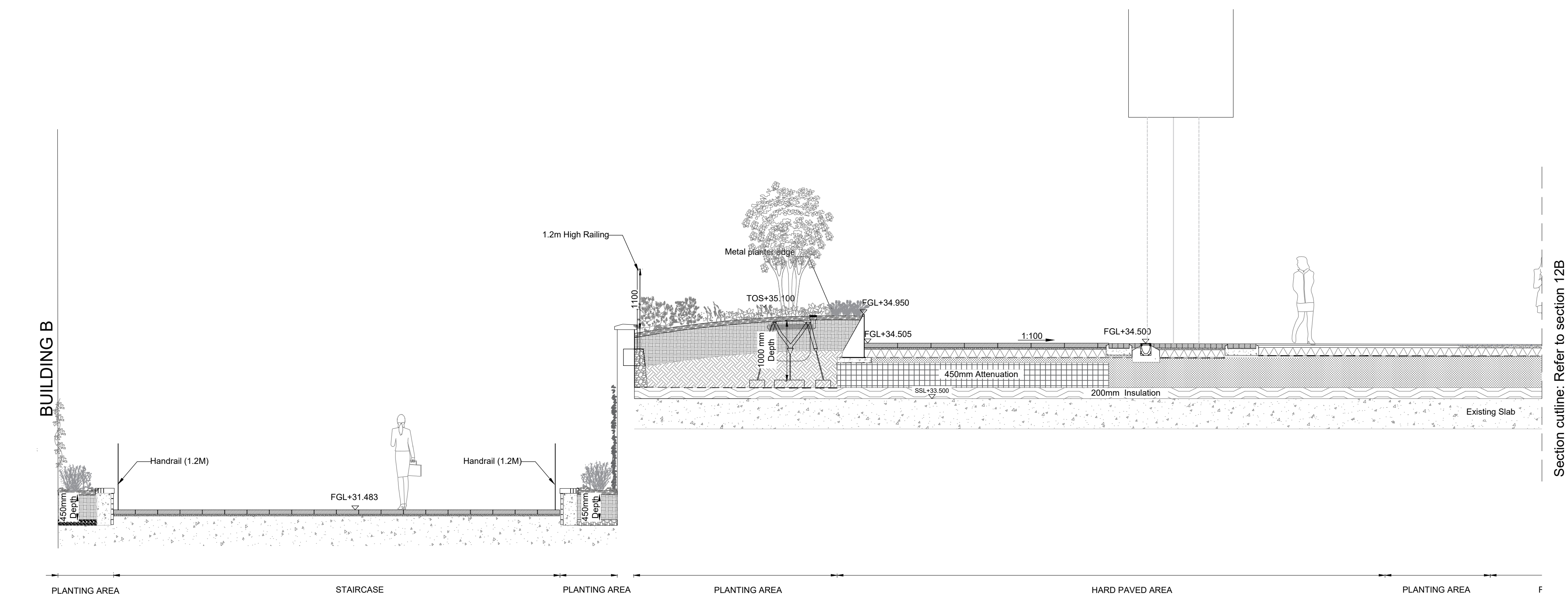
12A Stairs (Mid Point) to Railway Park Scale: 1:70
