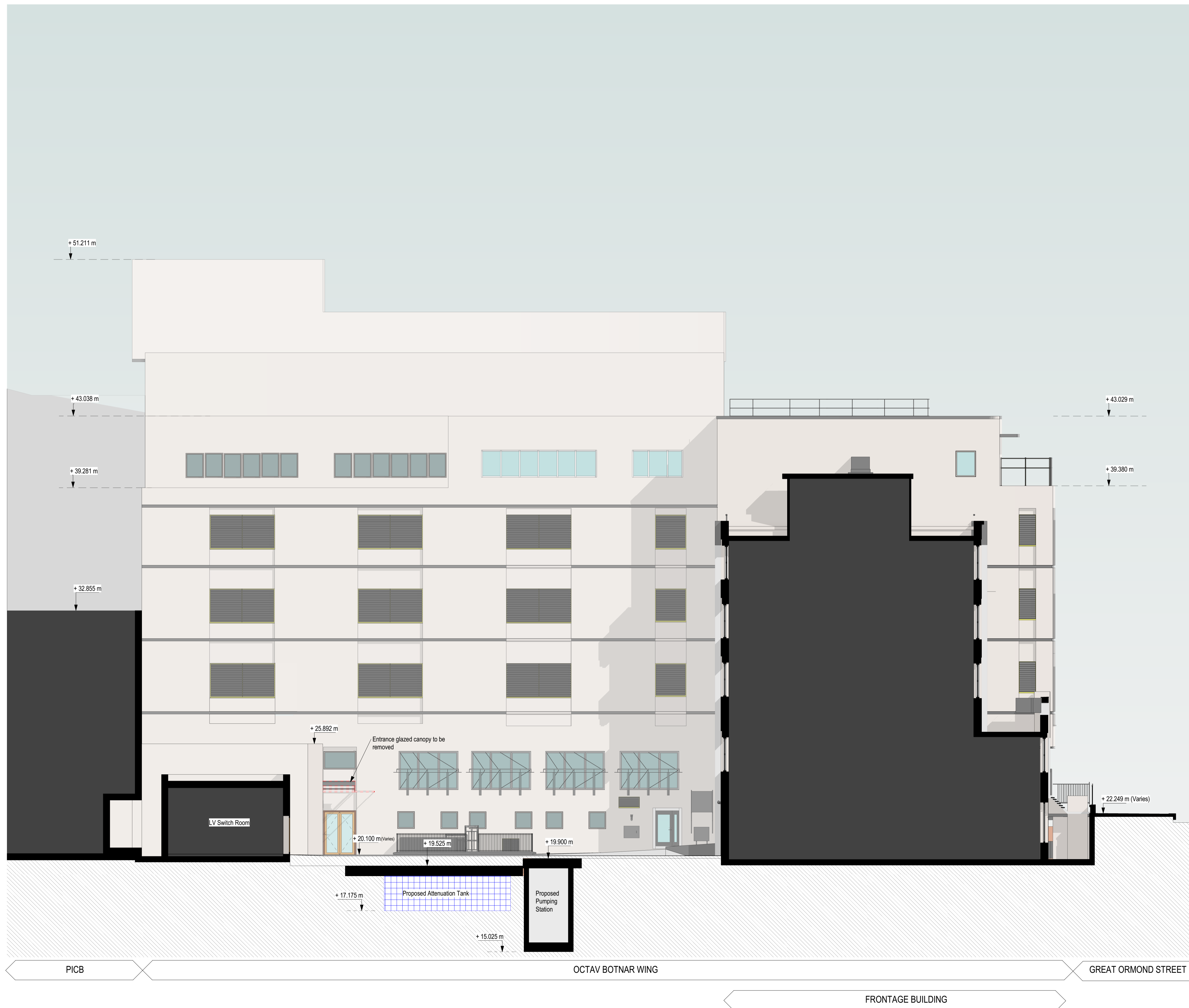
1 West Facing Sectional Elevation - Enabling Works 1 : 100
