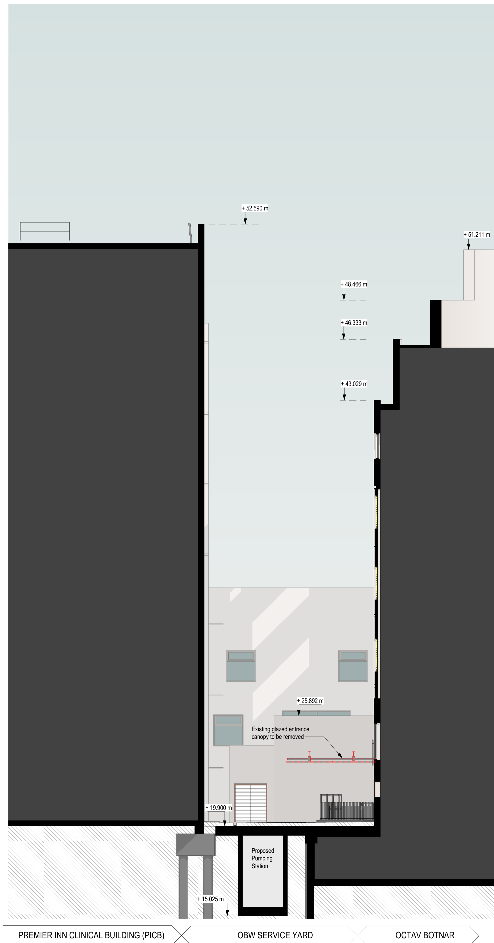
1 South Facing sectional Elevation - Enabling Works
