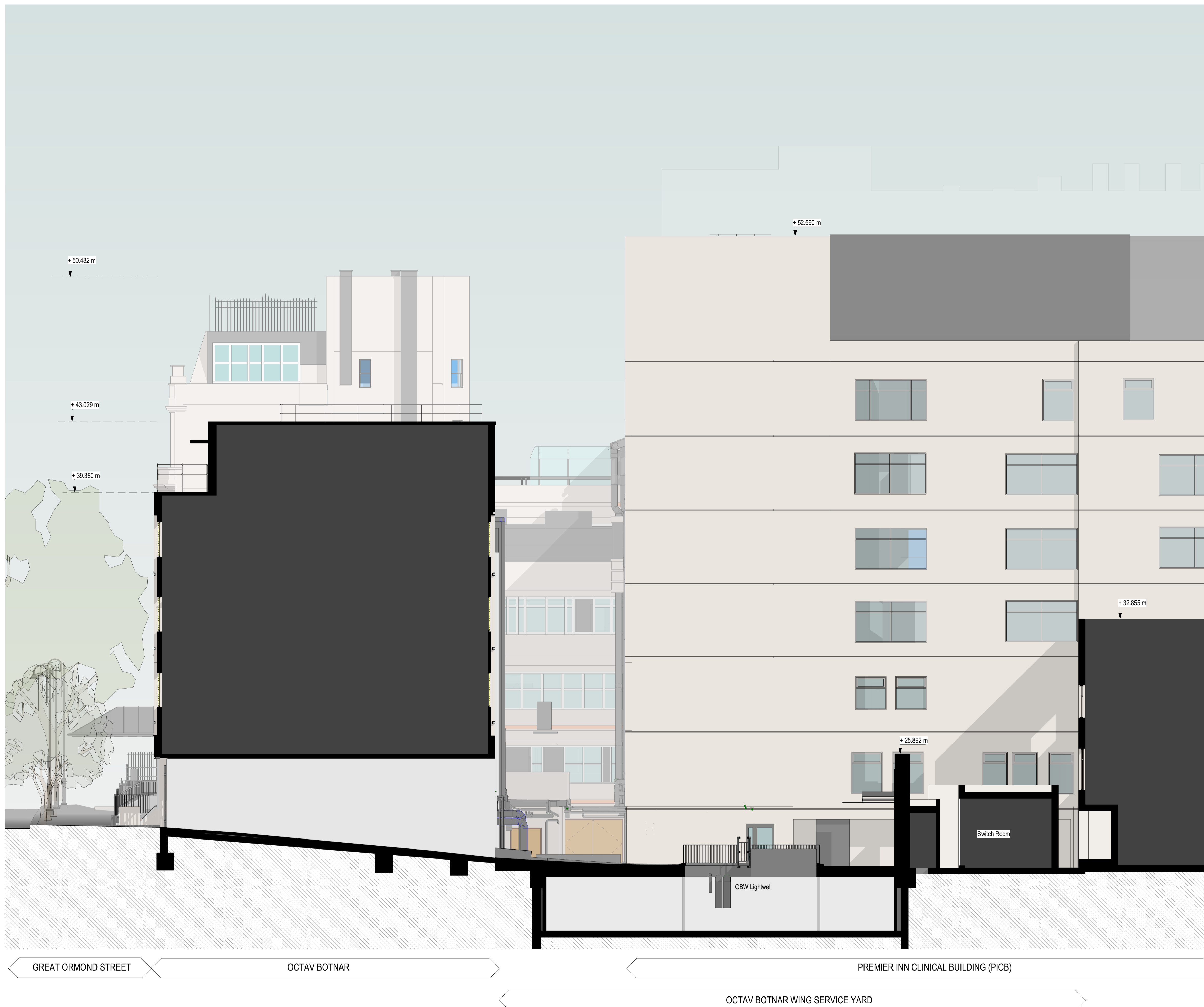
1 East Facing sectional Elevation as Existing 1 : 100
