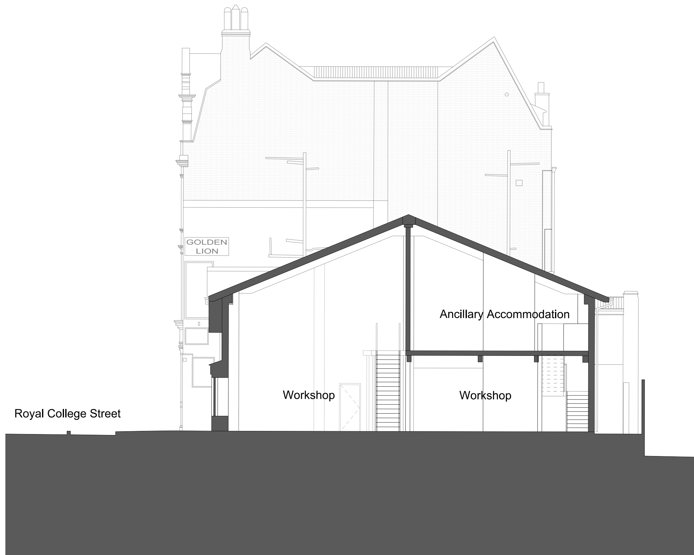
Section AA
