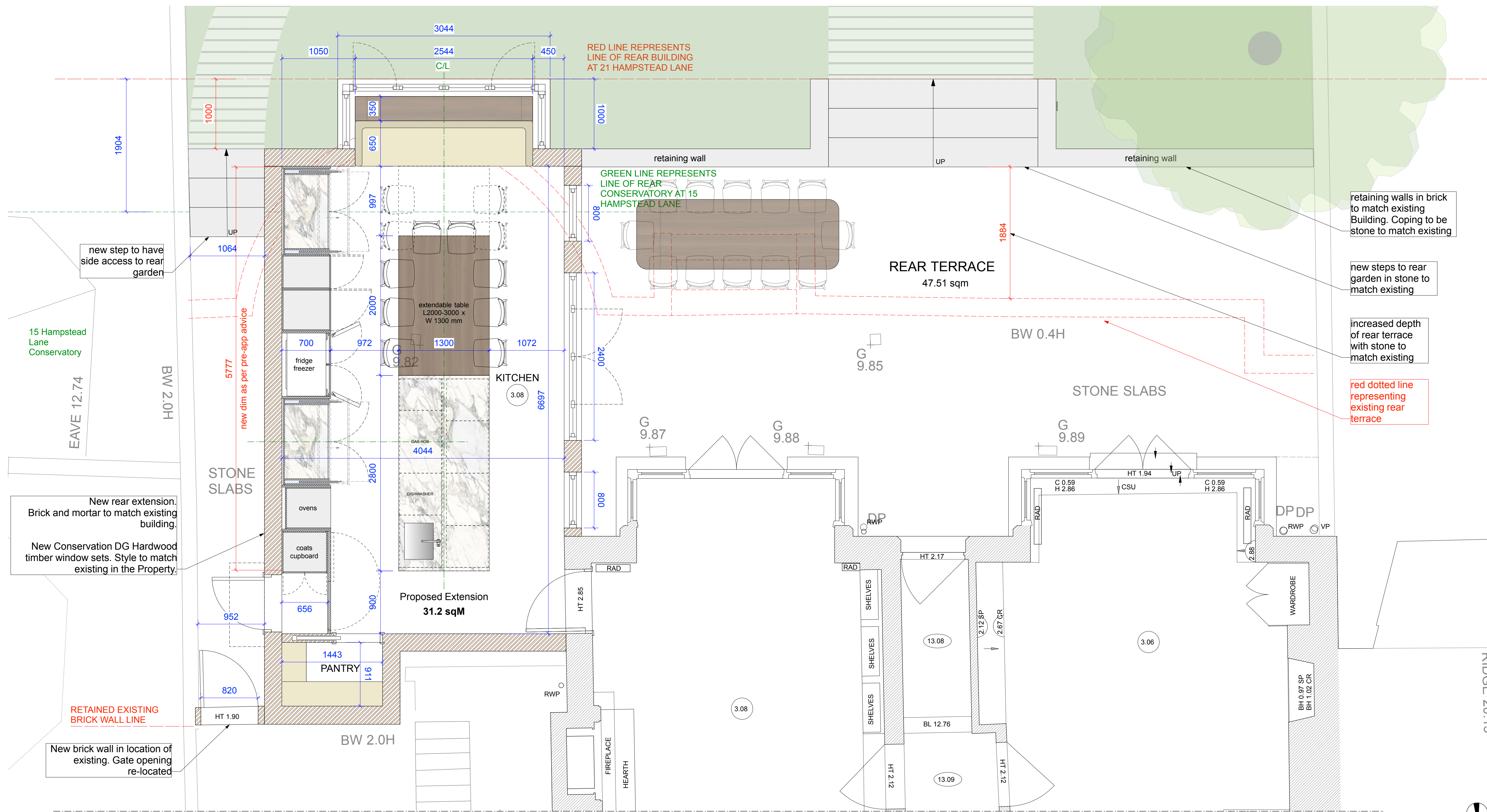
1 Rear Extension - Plan
