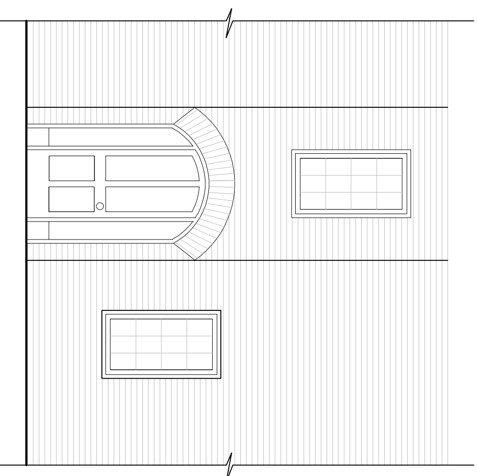
South-West Elevation
