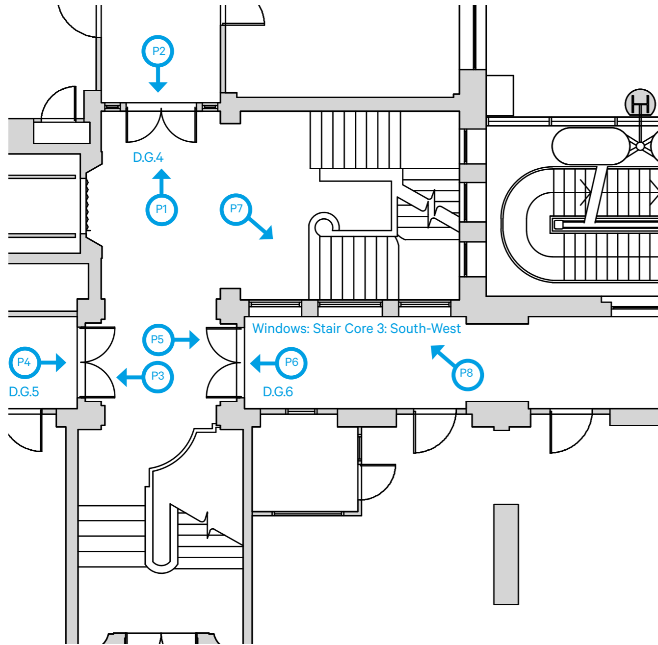
Plan of Stair Core 3: Ground Floor
