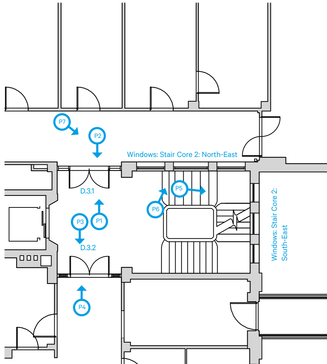
Plan of Stair Core 2: Third Floor
