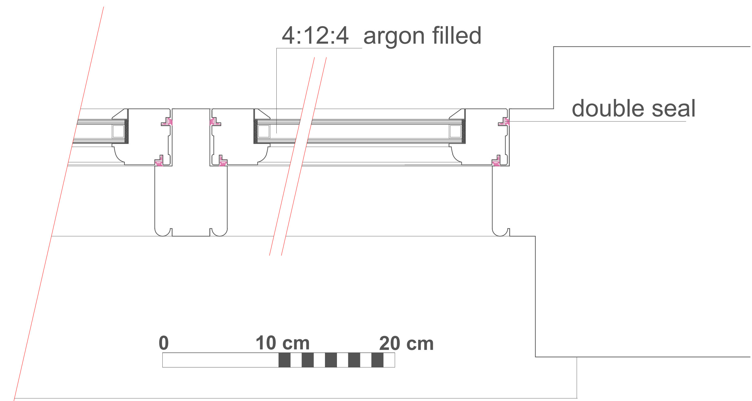
Proposed East elevation windows details 1:2
