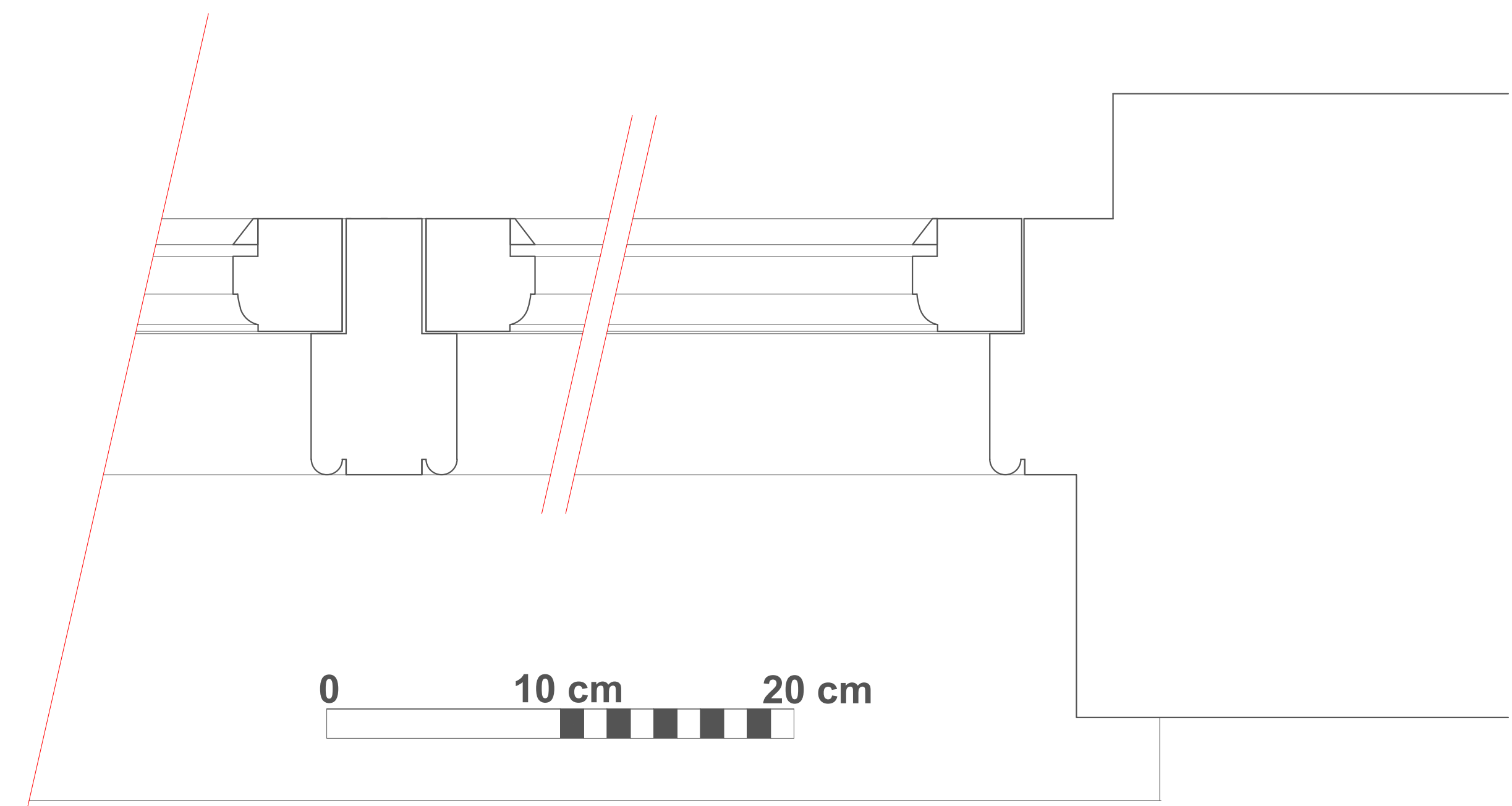
Existing East elevation window details 1:2
